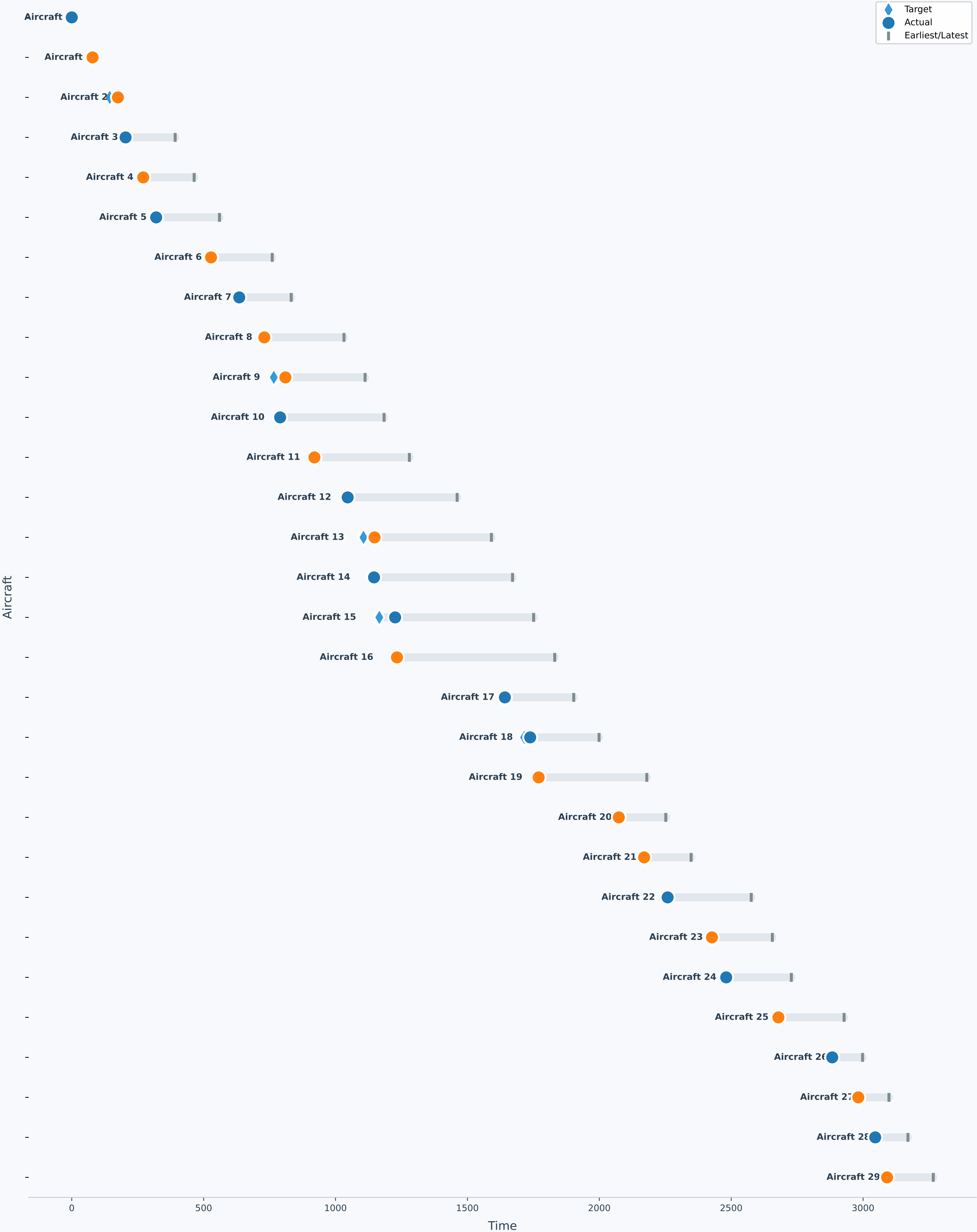
Schedule Details -- Instance 6 | 2 Runways | total_time | MIP
