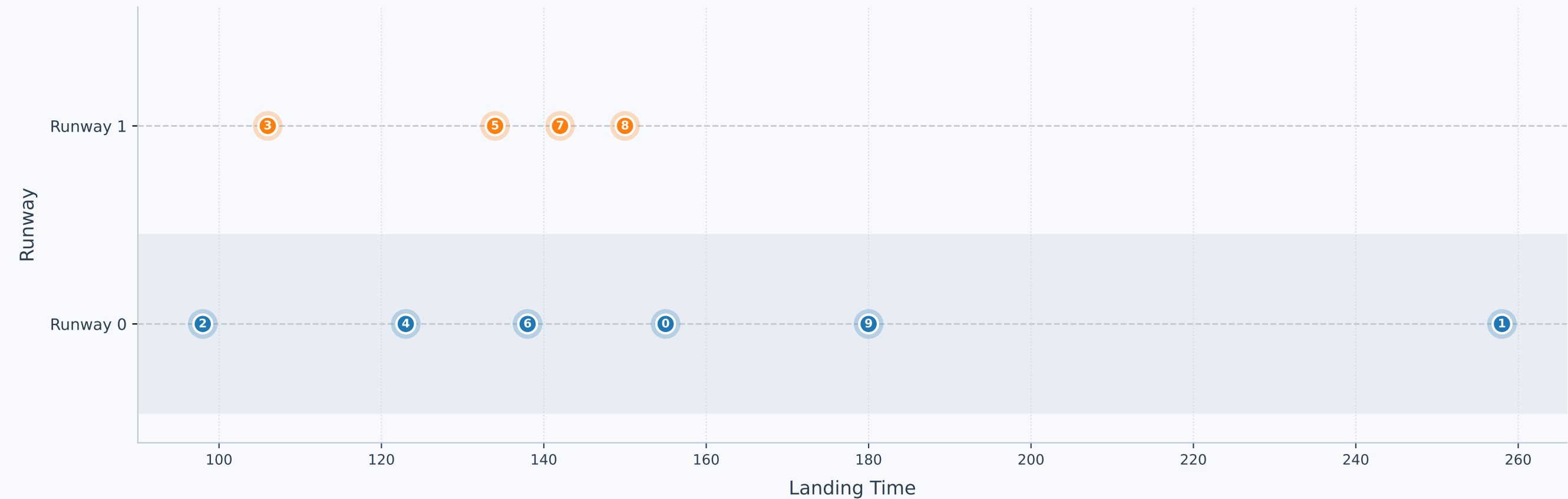
Landing Schedule -- Instance 1 | 2 Runways | penalty | MIP
