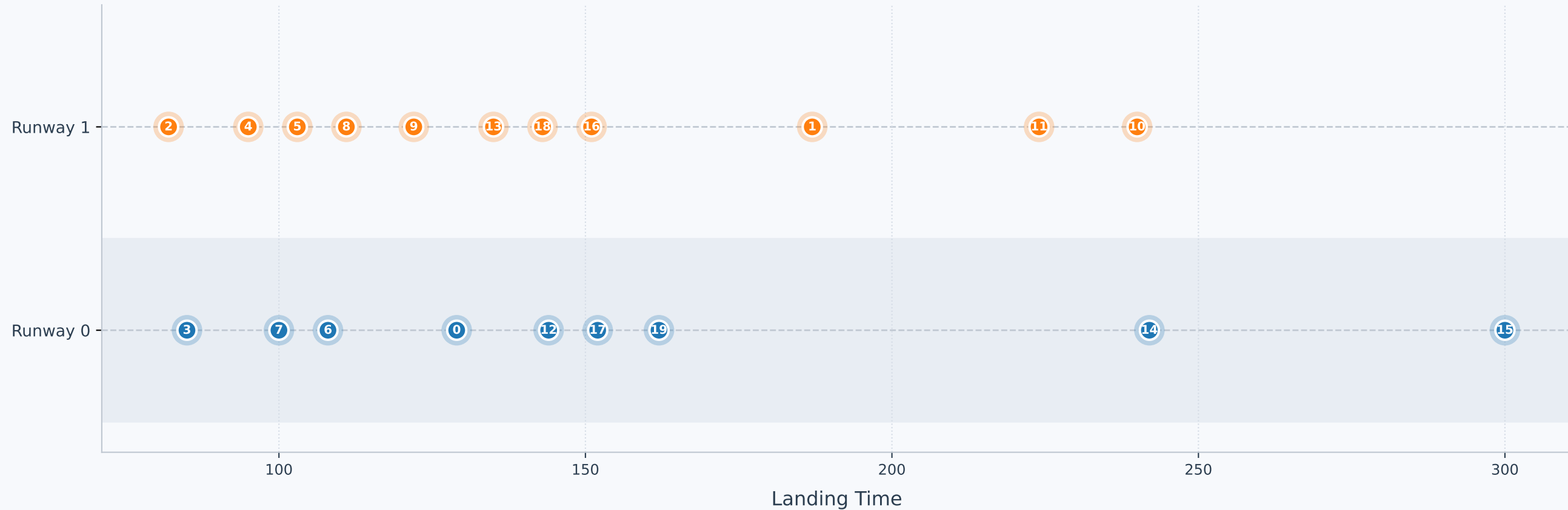
Landing Schedule -- Instance 5 | 2 Runways | total_time | MIP
