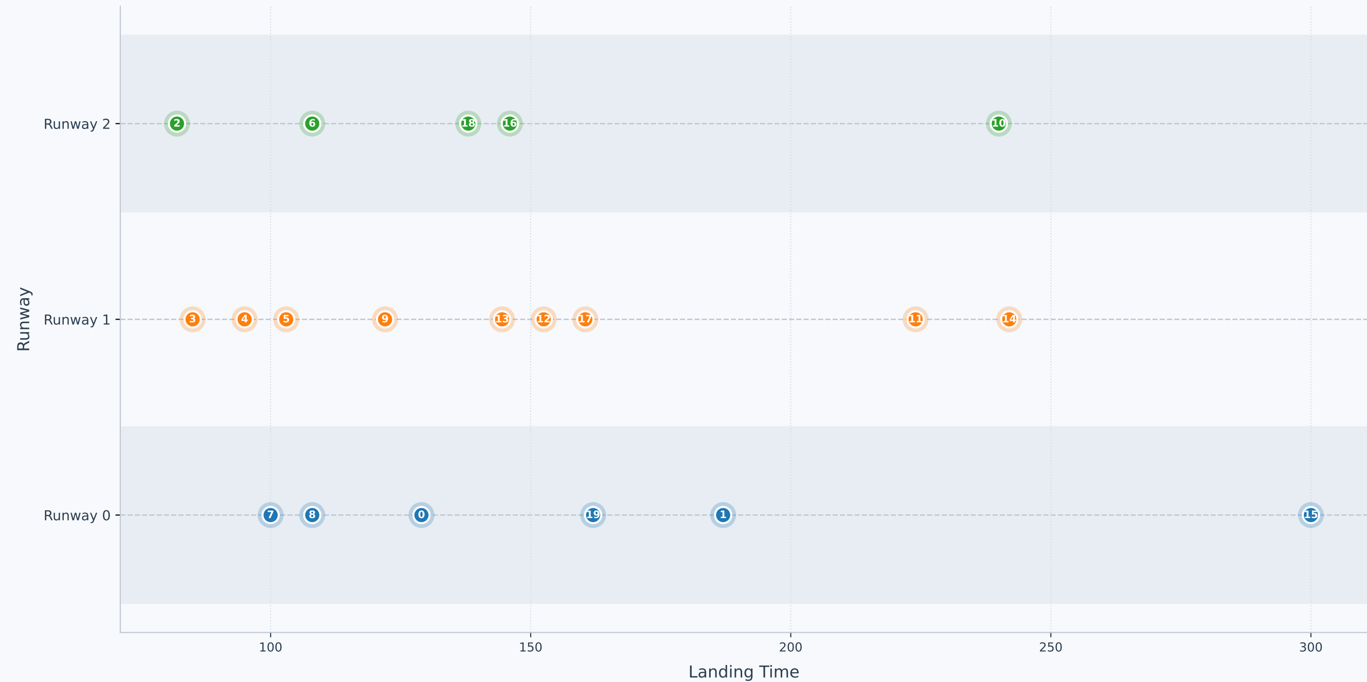
Landing Schedule -- Instance 5 | 3 Runways | makespan | MIP
