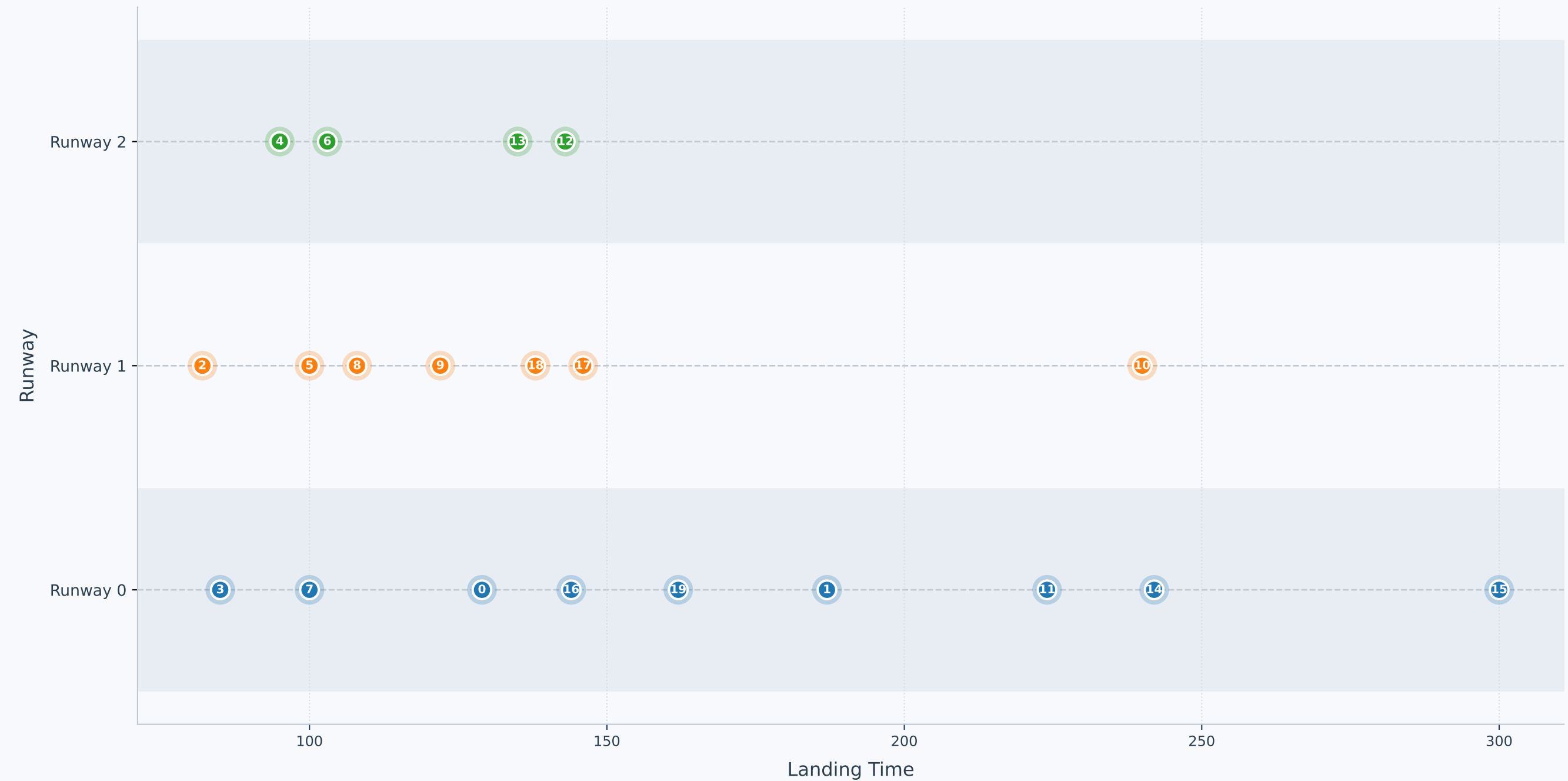
Landing Schedule -- Instance 5 | 3 Runways | total_time | MIP
