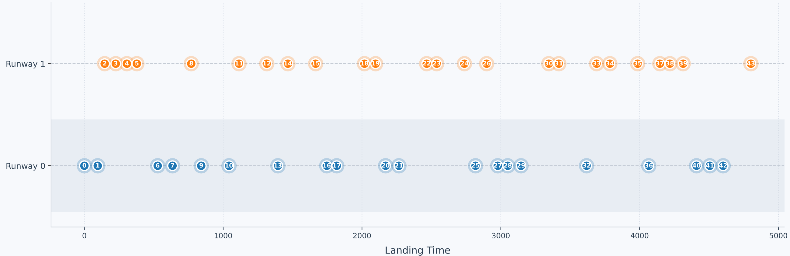
Landing Schedule -- Instance 7 | 2 Runways | total_time | MIP
