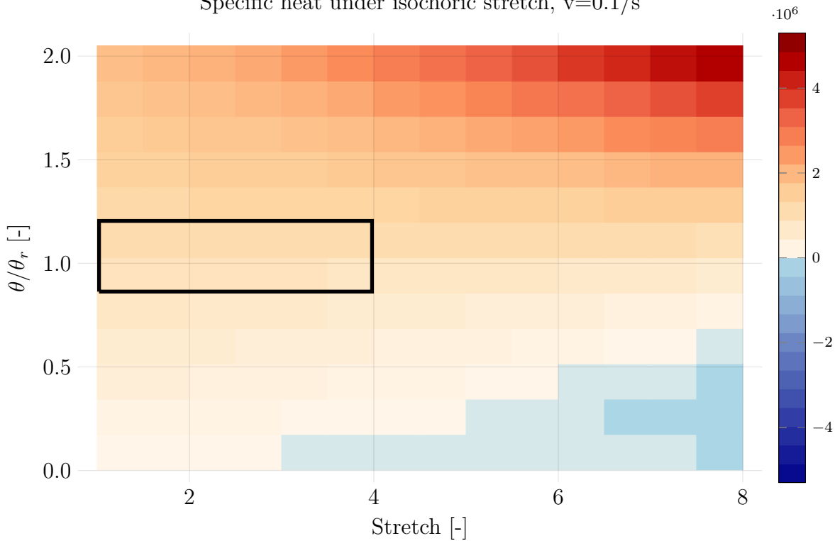
Specific heat under isochoric stretch, v=0.1/s
