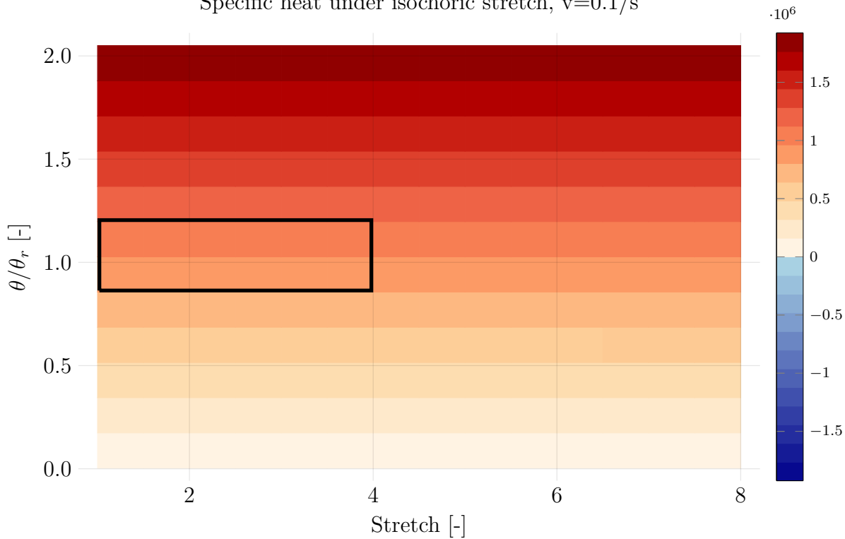
Specific heat under isochoric stretch, v=0.1/s
