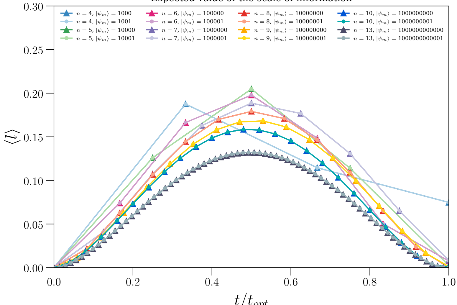
Expected value of the scale of information
