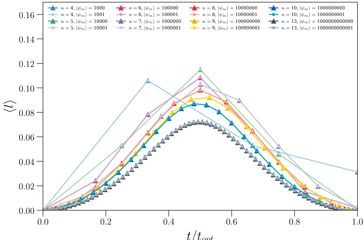
Median of the scale of information
