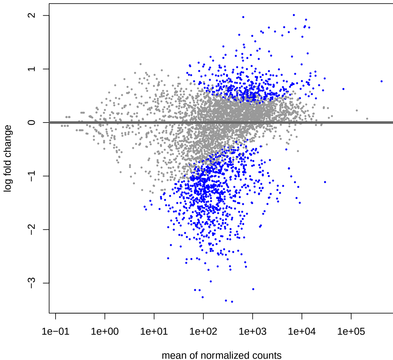
MA-plot for Gene_Type: WildType vs Mutants
