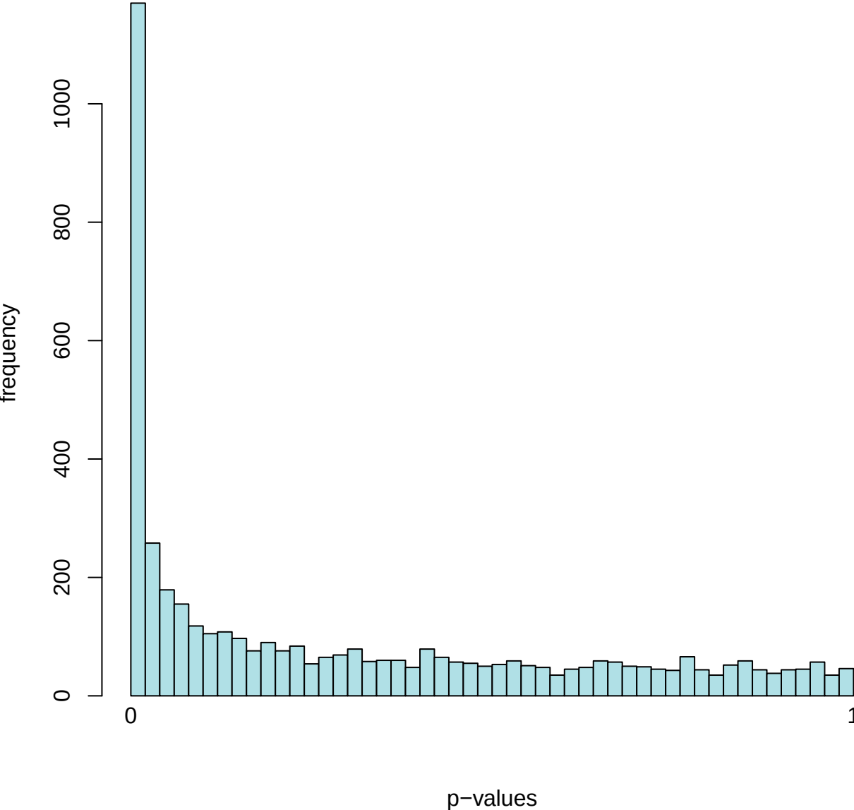
Histogram of p-values for Gene_Type: WildType vs Mutants
