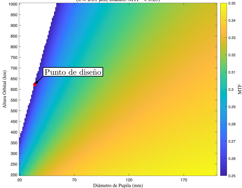
MTF - Refractivo - Detector 2 ( \lambda = 2.01 \mu\text{m} , Blanco: MTF < 0.25)
