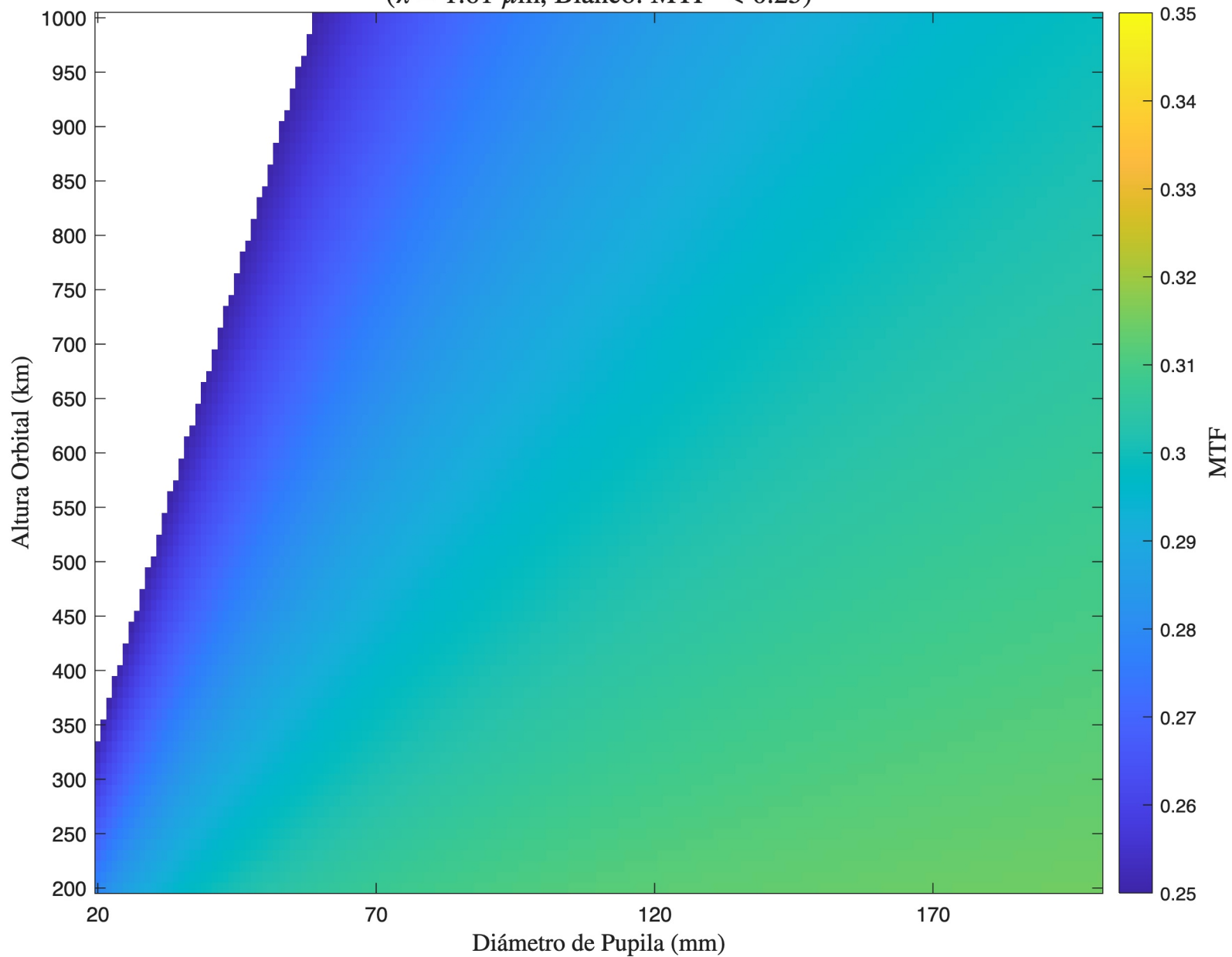
MTF - Refractivo - Detector 1 ( \lambda = 1.61 \mu\text{m} , Blanco: MTF < 0.25)
