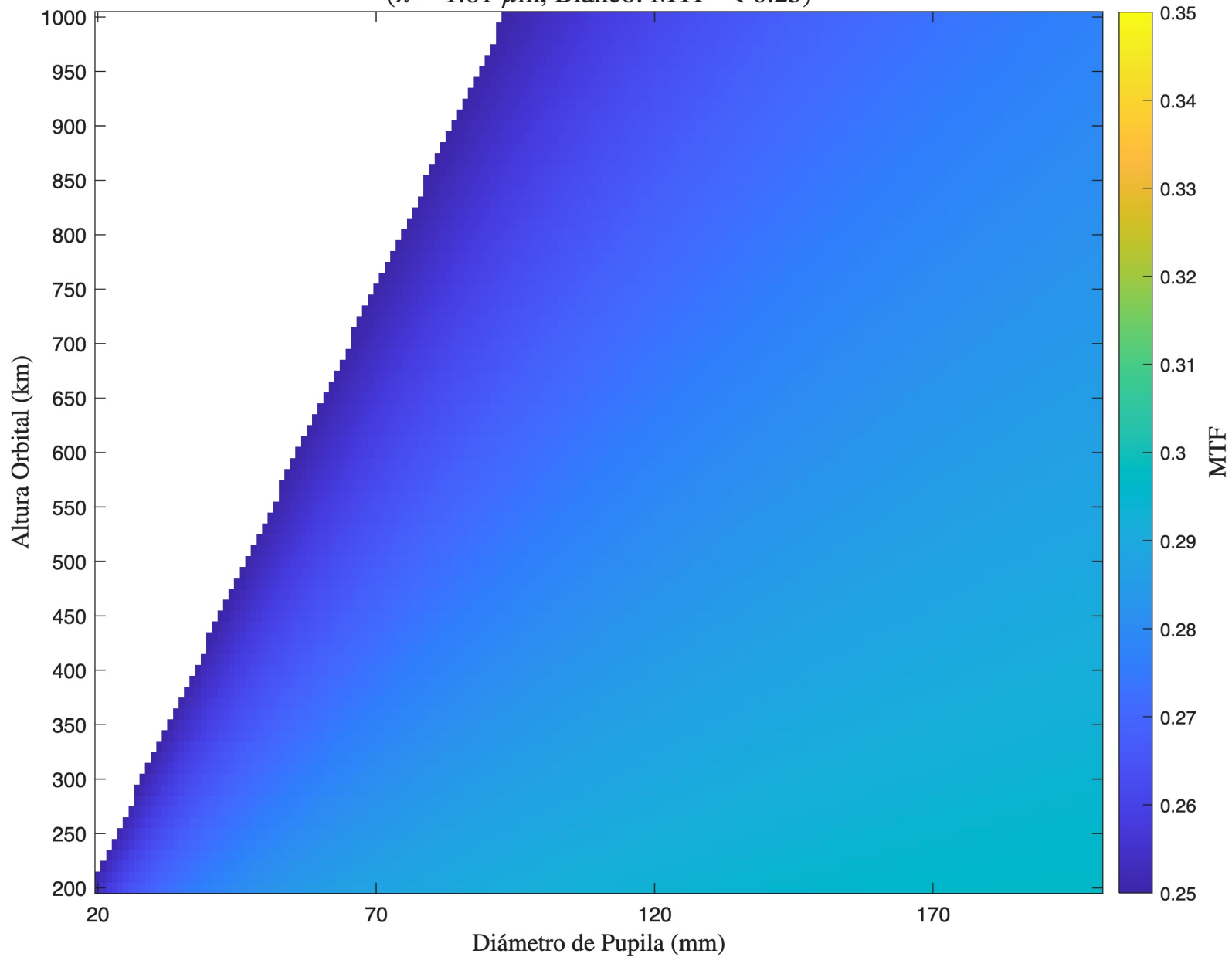
MTF - Korsch - Detector 1 ( \lambda = 1.61 \mu\text{m} , Blanco: MTF < 0.25)
