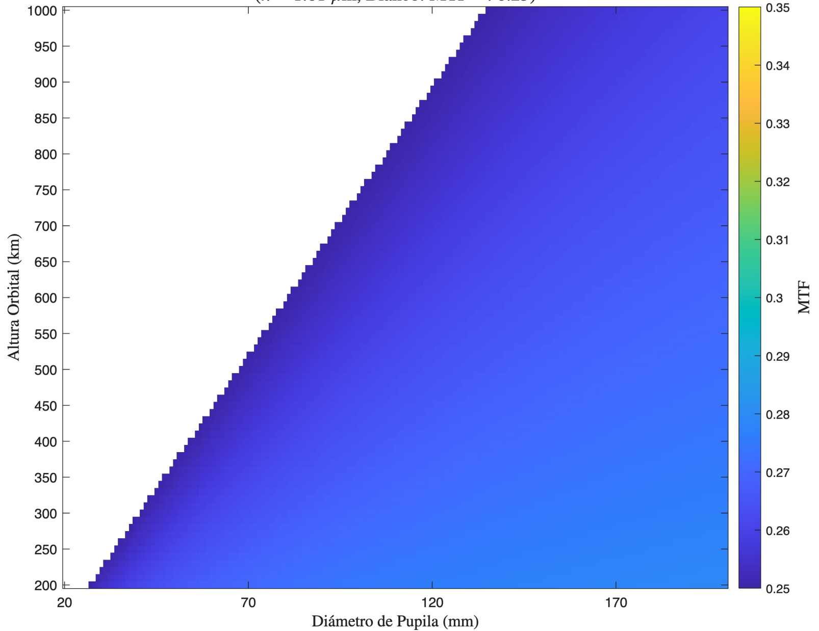
MTF - Cassegrain - Detector 1 ( \lambda = 1.61 \mu\text{m} , Blanco: MTF < 0.25)
