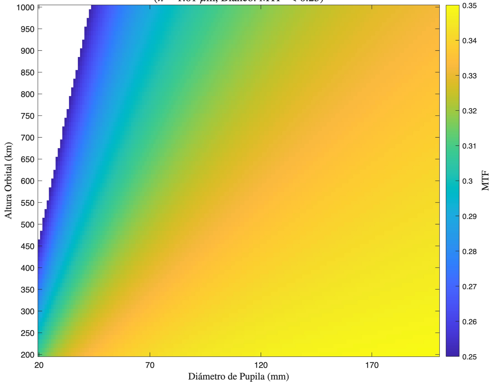
MTF - Refractivo - Detector 2 ( \lambda = 1.61 \mu\text{m} , Blanco: MTF < 0.25)
