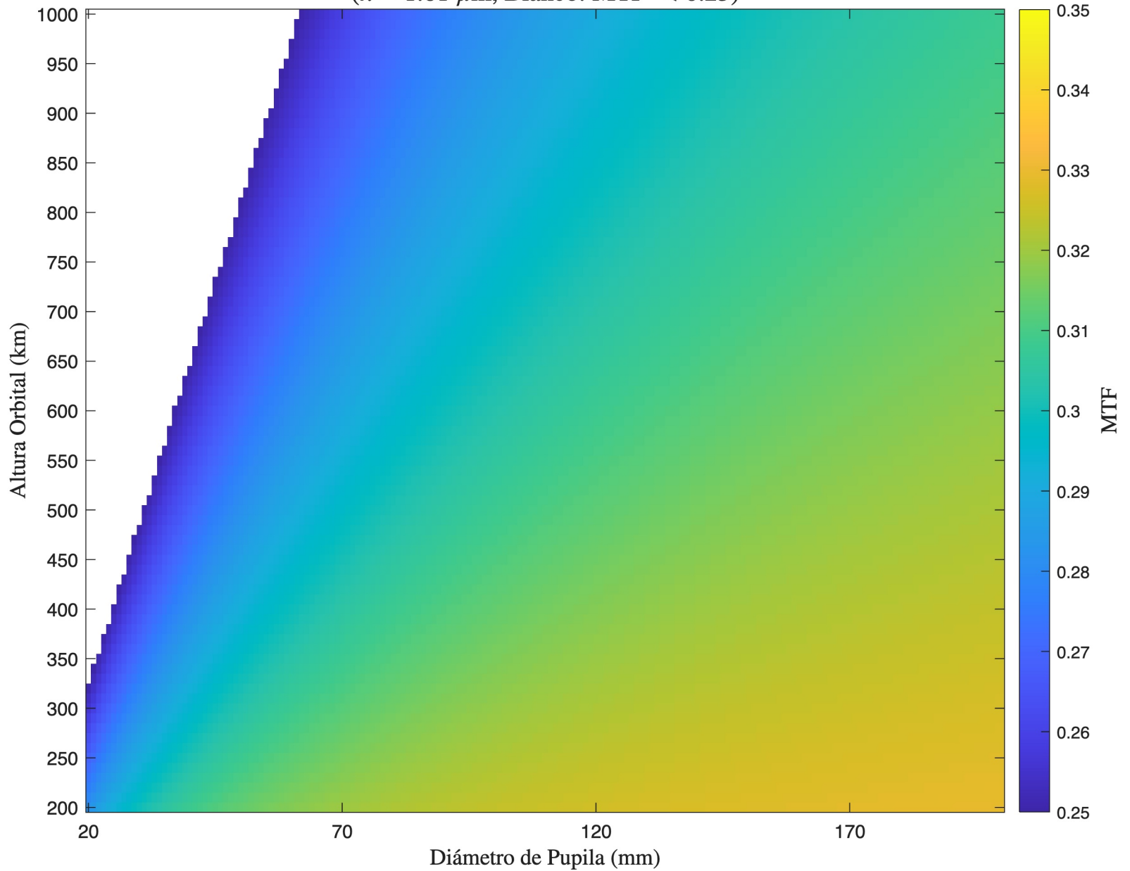
MTF - Korsch - Detector 2 ( \lambda = 1.61 \mu\text{m} , Blanco: MTF < 0.25)
