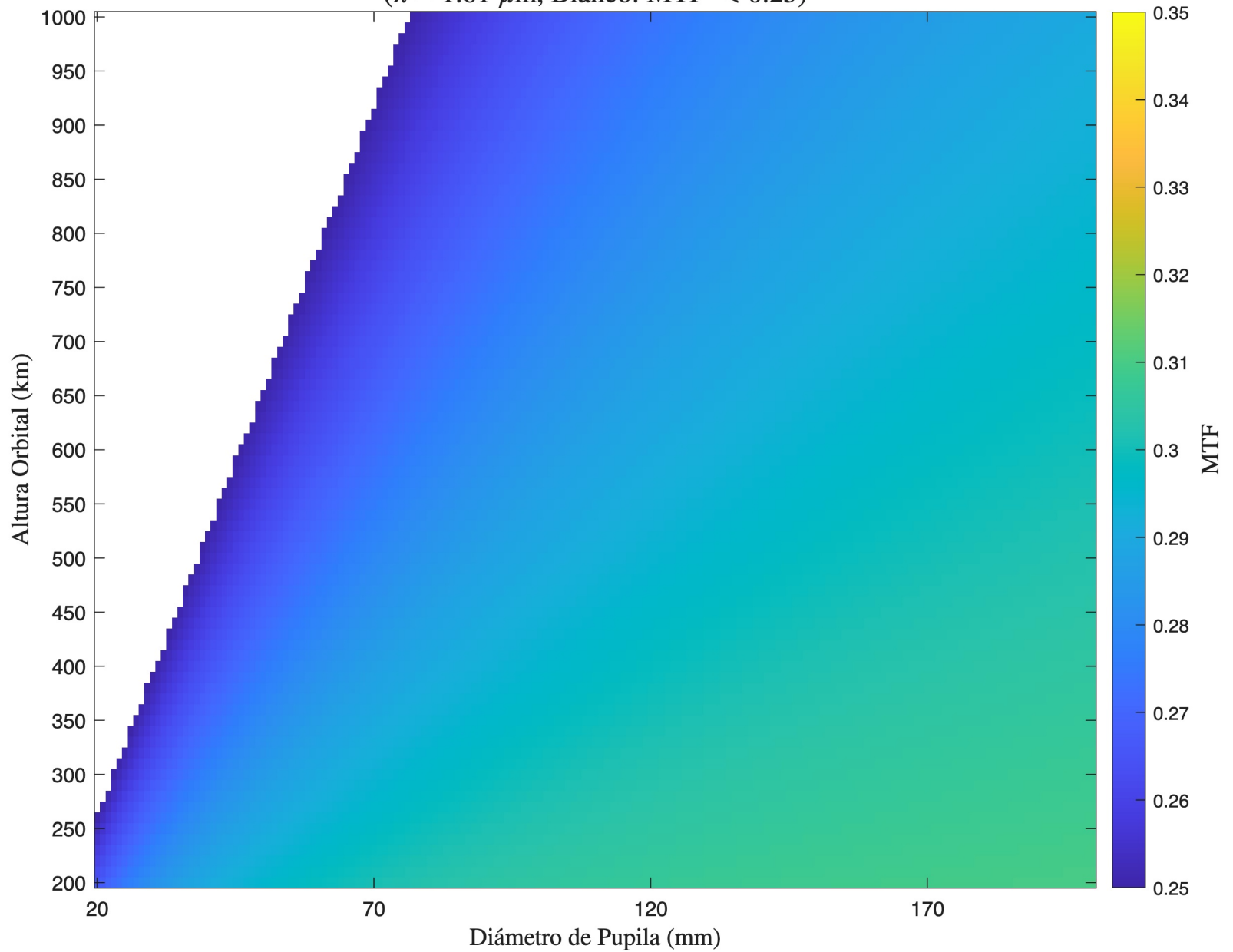
MTF - Cassegrain - Detector 2 ( \lambda = 1.61 \mu\text{m} , Blanco: MTF < 0.25)
