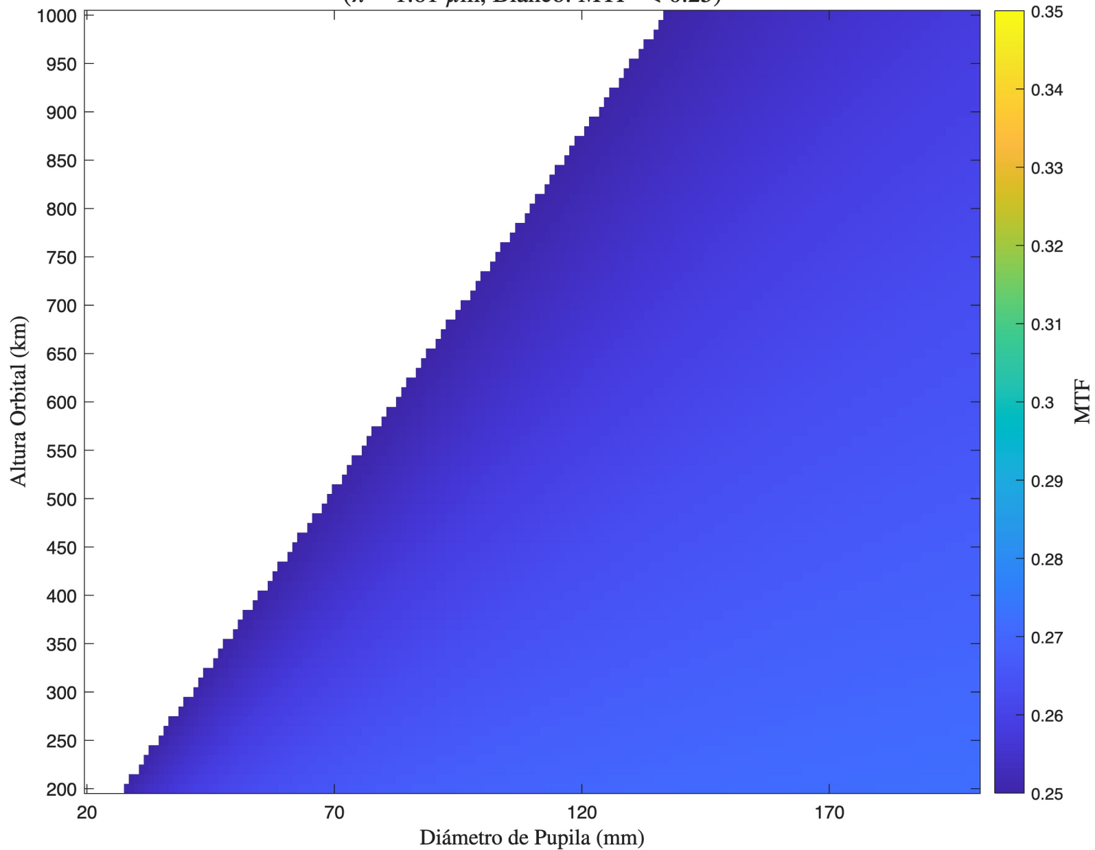
MTF - TMA - Detector 2 ( \lambda = 1.61 \mu\text{m} , Blanco: MTF < 0.25)
