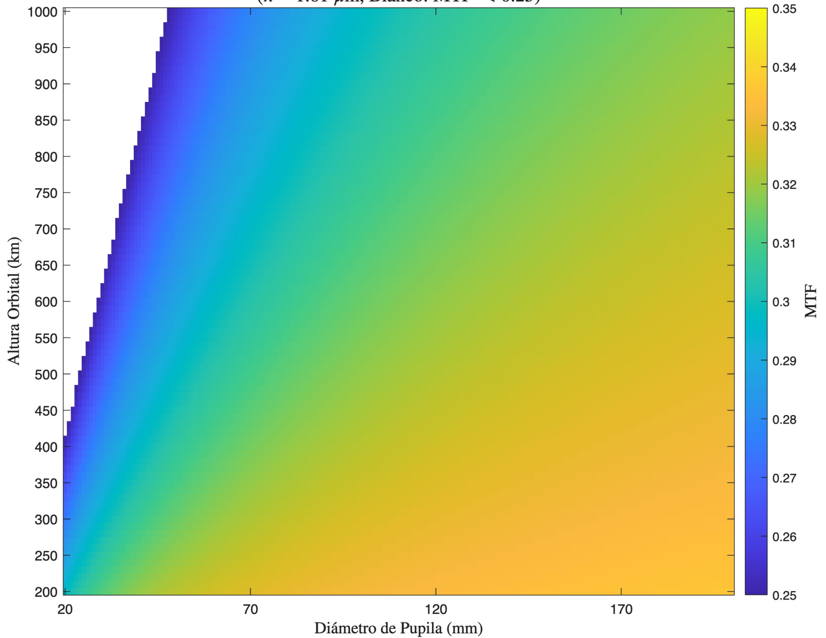
MTF - Refractivo - Detector 3 ( \lambda = 1.61 \mu\text{m} , Blanco: MTF < 0.25)
