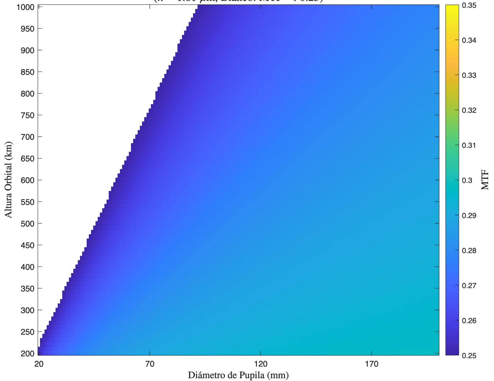
MTF - Cassegrain - Detector 3 ( \lambda = 1.61 \mu\text{m} , Blanco: MTF < 0.25)
