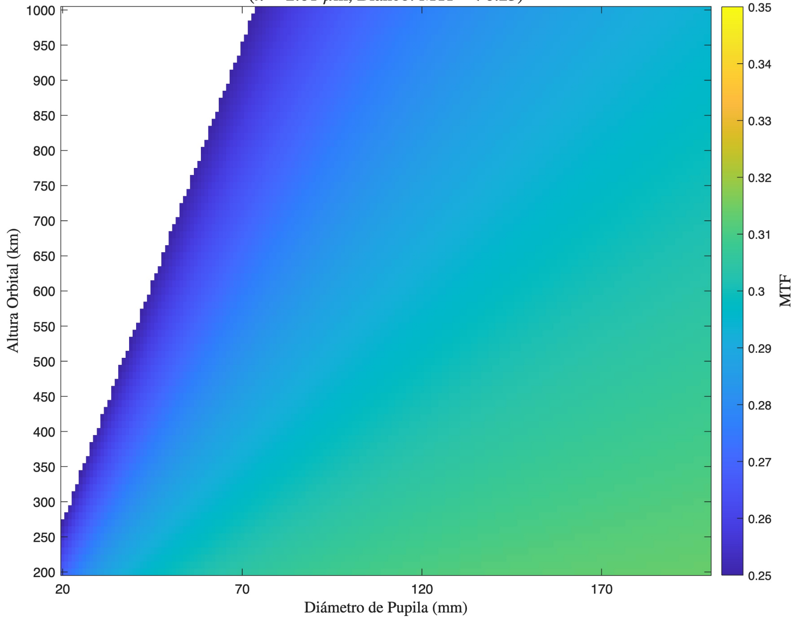
MTF - Refractivo - Detector 1 ( \lambda = 2.01 \mu\text{m} , Blanco: MTF < 0.25)
