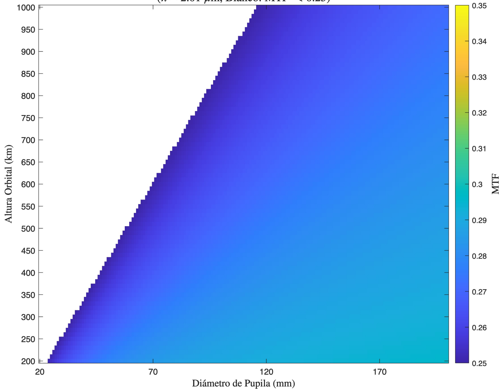
MTF - Korsch - Detector 1 ( \lambda = 2.01 \mu\text{m} , Blanco: MTF < 0.25)
