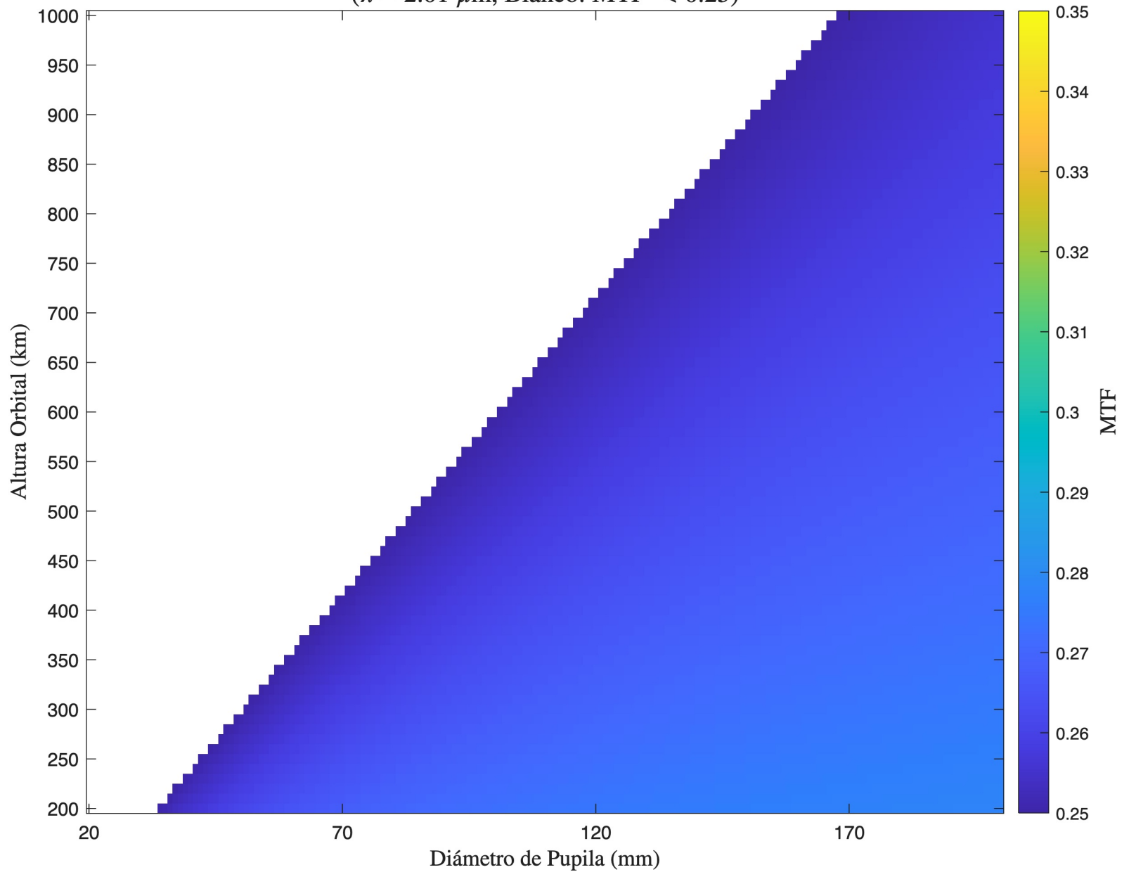
MTF - Cassegrain - Detector 1 ( \lambda = 2.01 \mu\text{m} , Blanco: MTF < 0.25)
