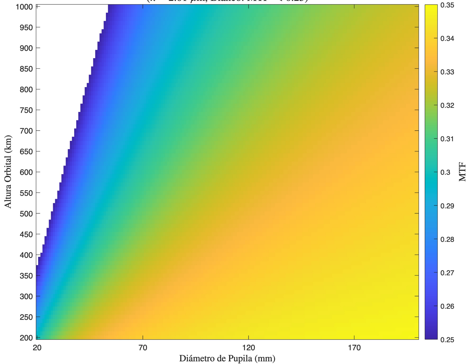
MTF - Refractivo - Detector 2 ( \lambda = 2.01 \mu\text{m} , Blanco: MTF < 0.25)
