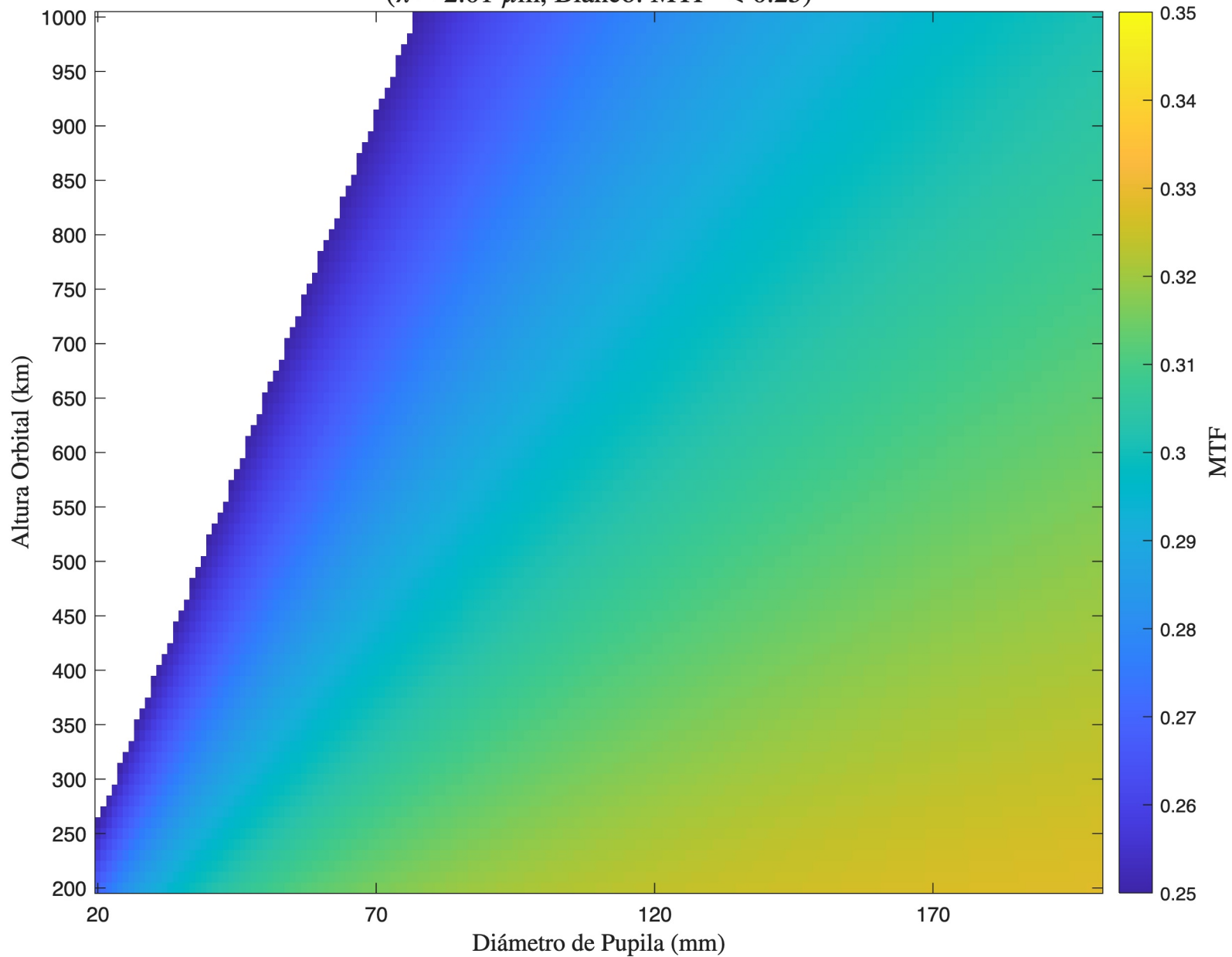
MTF - Korsch - Detector 2 ( \lambda = 2.01 \mu\text{m} , Blanco: MTF < 0.25)
