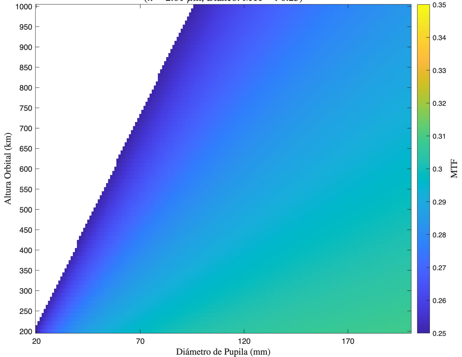
MTF - Cassegrain - Detector 2 ( \lambda = 2.01 \mu\text{m} , Blanco: MTF < 0.25)
