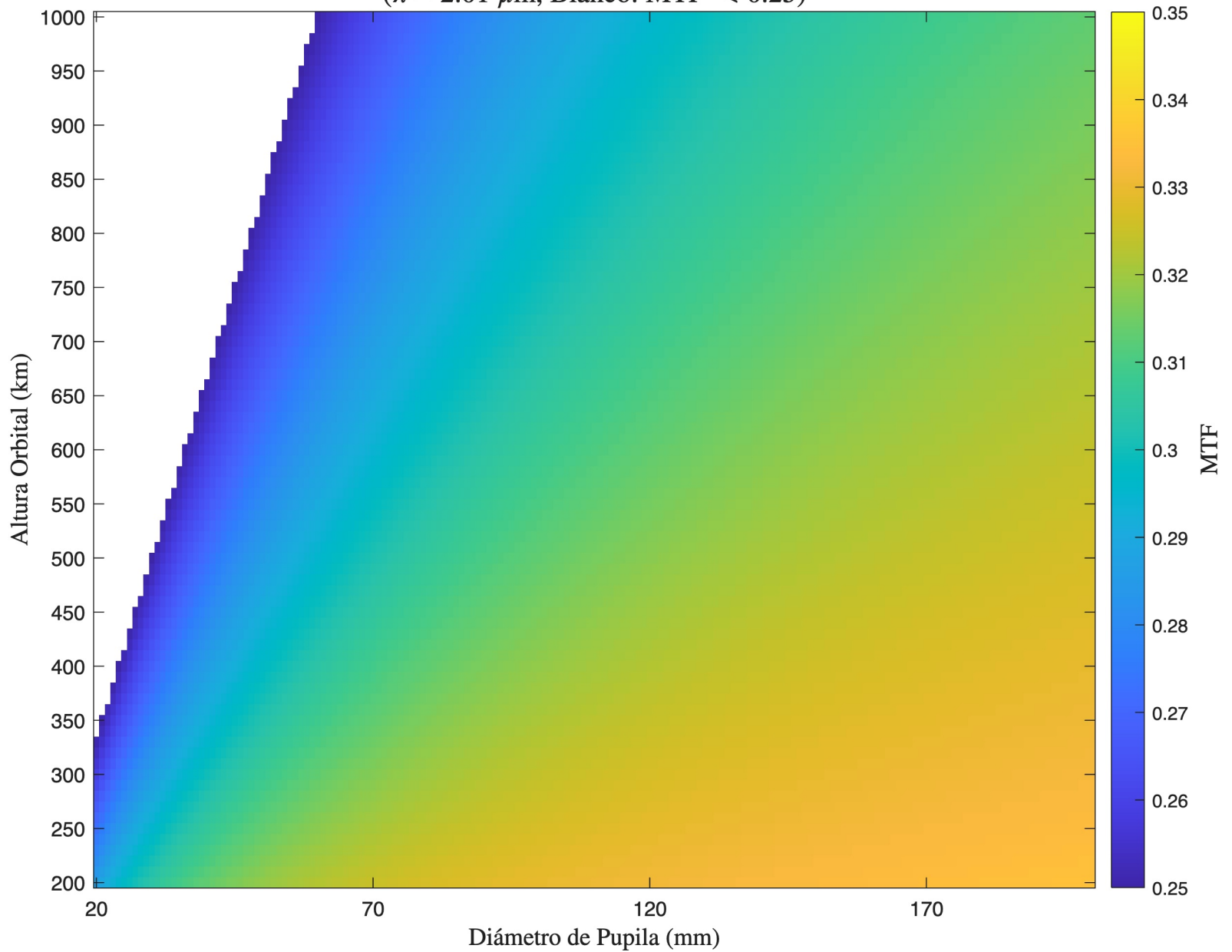
MTF - Refractivo - Detector 3 ( \lambda = 2.01 \mu\text{m} , Blanco: MTF < 0.25)
