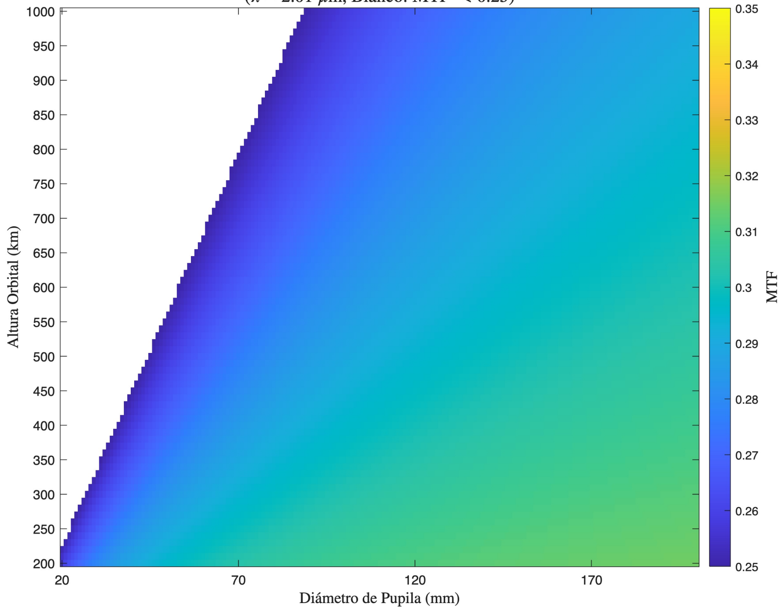
MTF - Korsch - Detector 3 ( \lambda = 2.01 \mu\text{m} , Blanco: MTF < 0.25)
