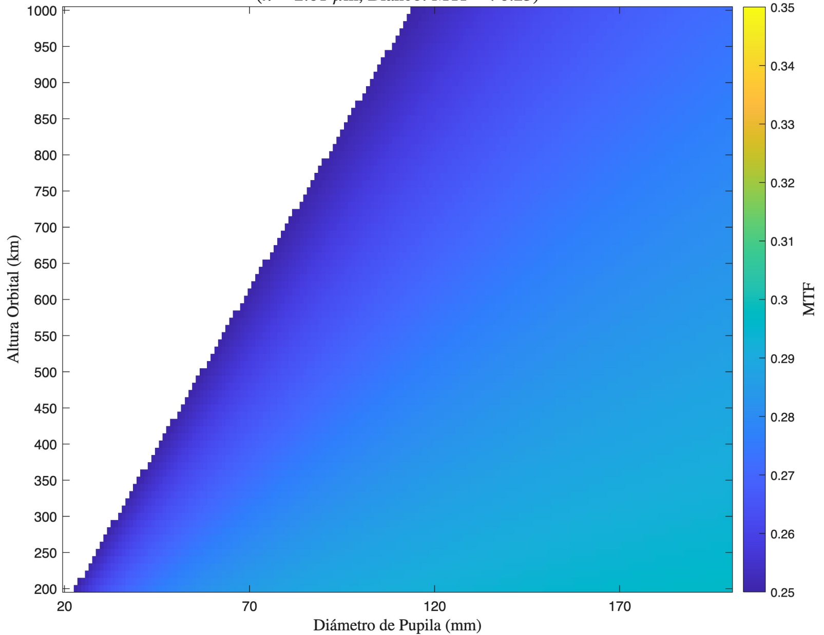
MTF - Cassegrain - Detector 3 ( \lambda = 2.01 \mu\text{m} , Blanco: MTF < 0.25)
