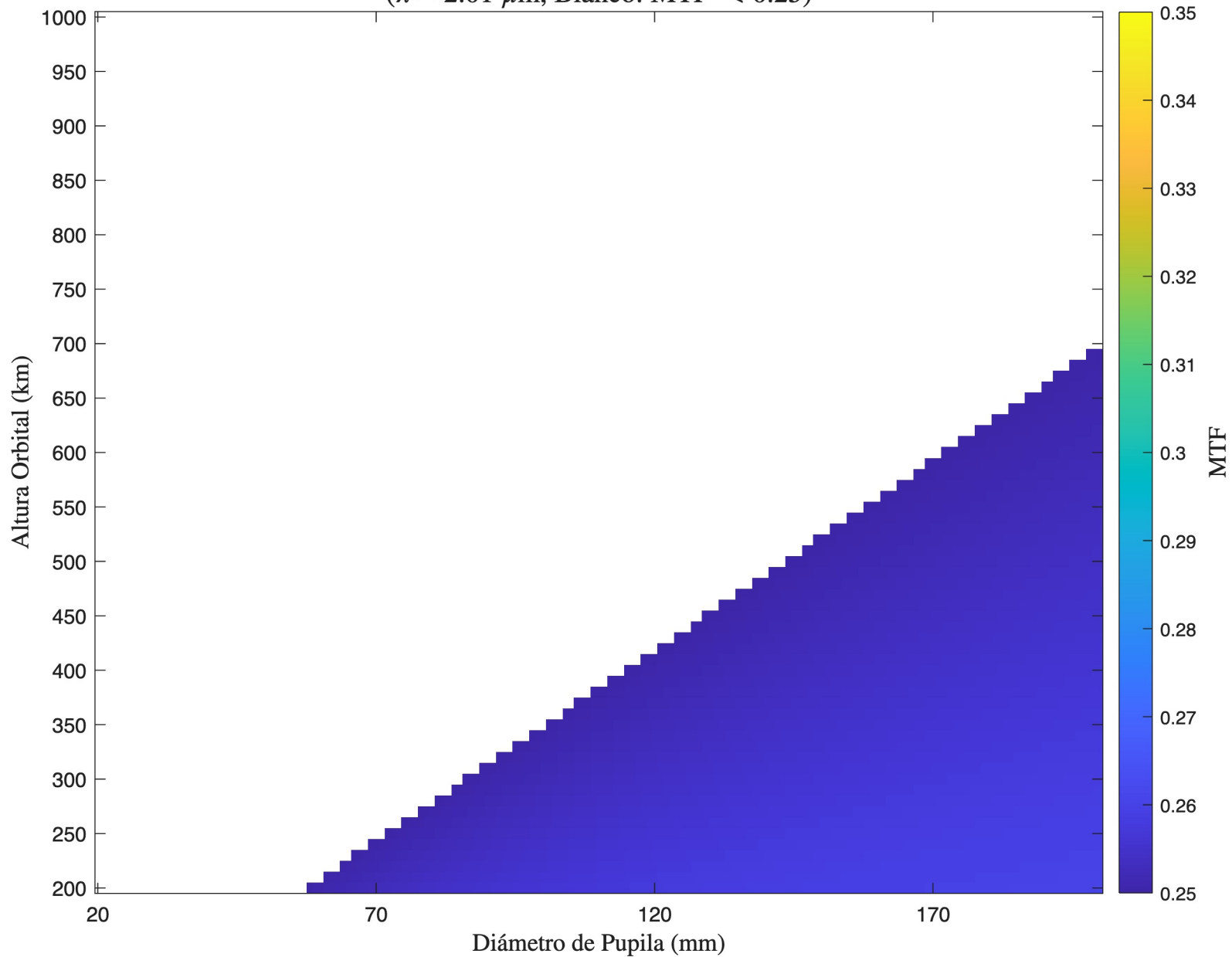
MTF - TMA - Detector 3 ( \lambda = 2.01 \mu\text{m} , Blanco: MTF < 0.25)
