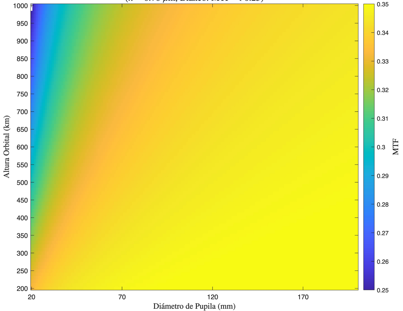
MTF - Refractivo - Detector 1 ( \lambda = 0.76 \mu\text{m} , Blanco: MTF < 0.25)
