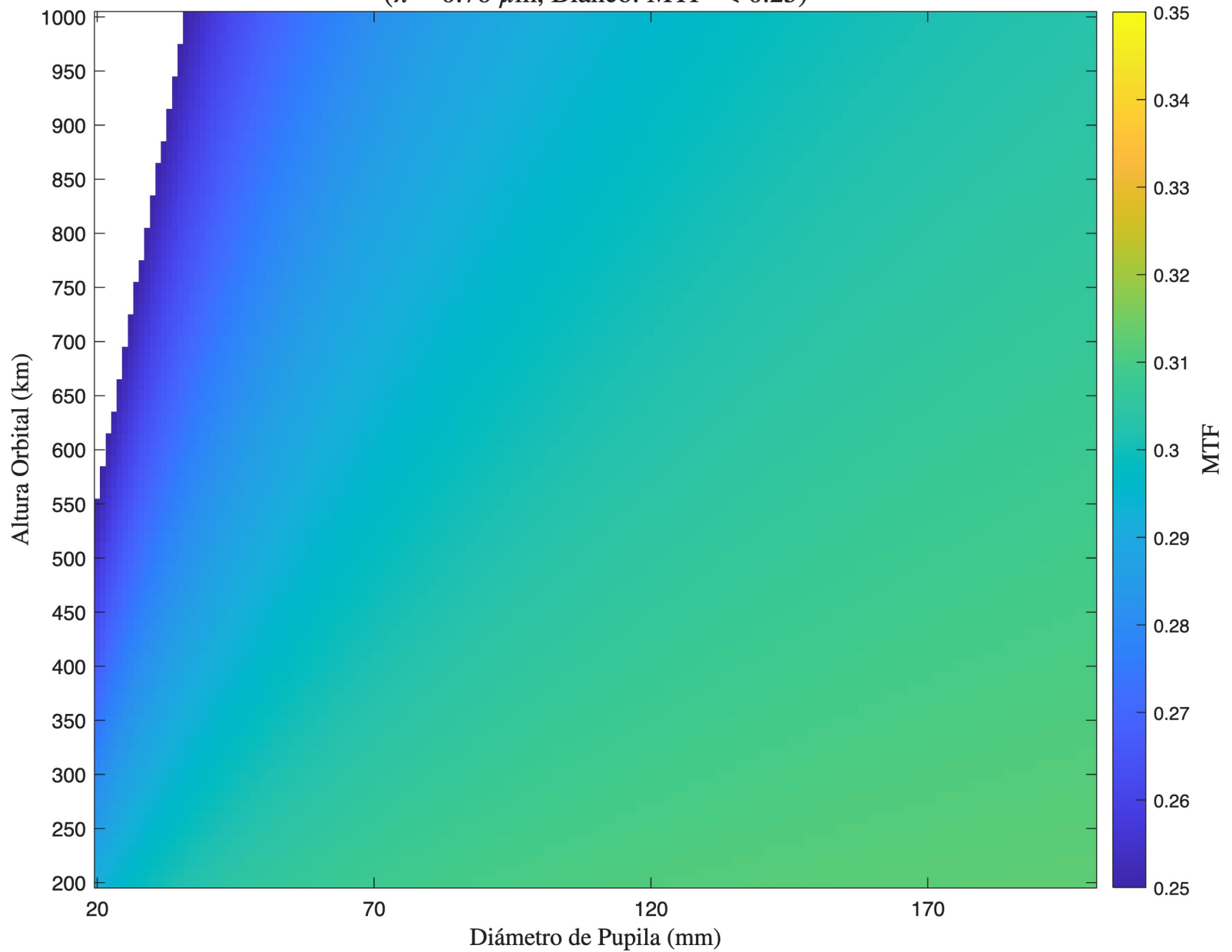
MTF - Cassegrain - Detector 1 ( \lambda = 0.76 \mu\text{m} , Blanco: MTF < 0.25)
