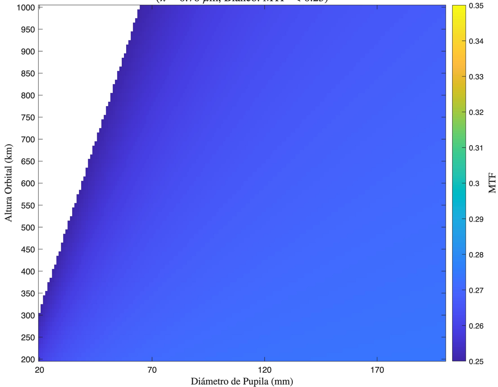
MTF - TMA - Detector 1 ( \lambda = 0.76 \mu\text{m} , Blanco: MTF < 0.25)
