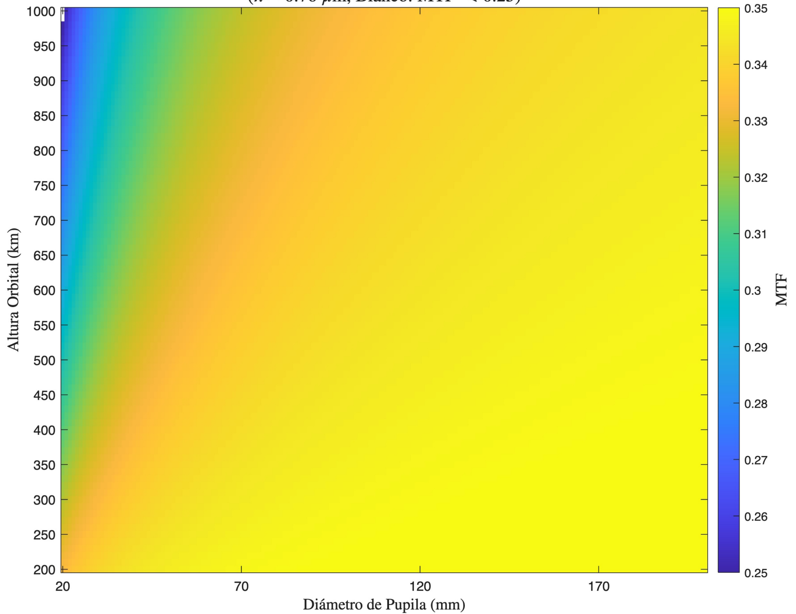
MTF - Refractivo - Detector 2 ( \lambda = 0.76 \mu\text{m} , Blanco: MTF < 0.25)
