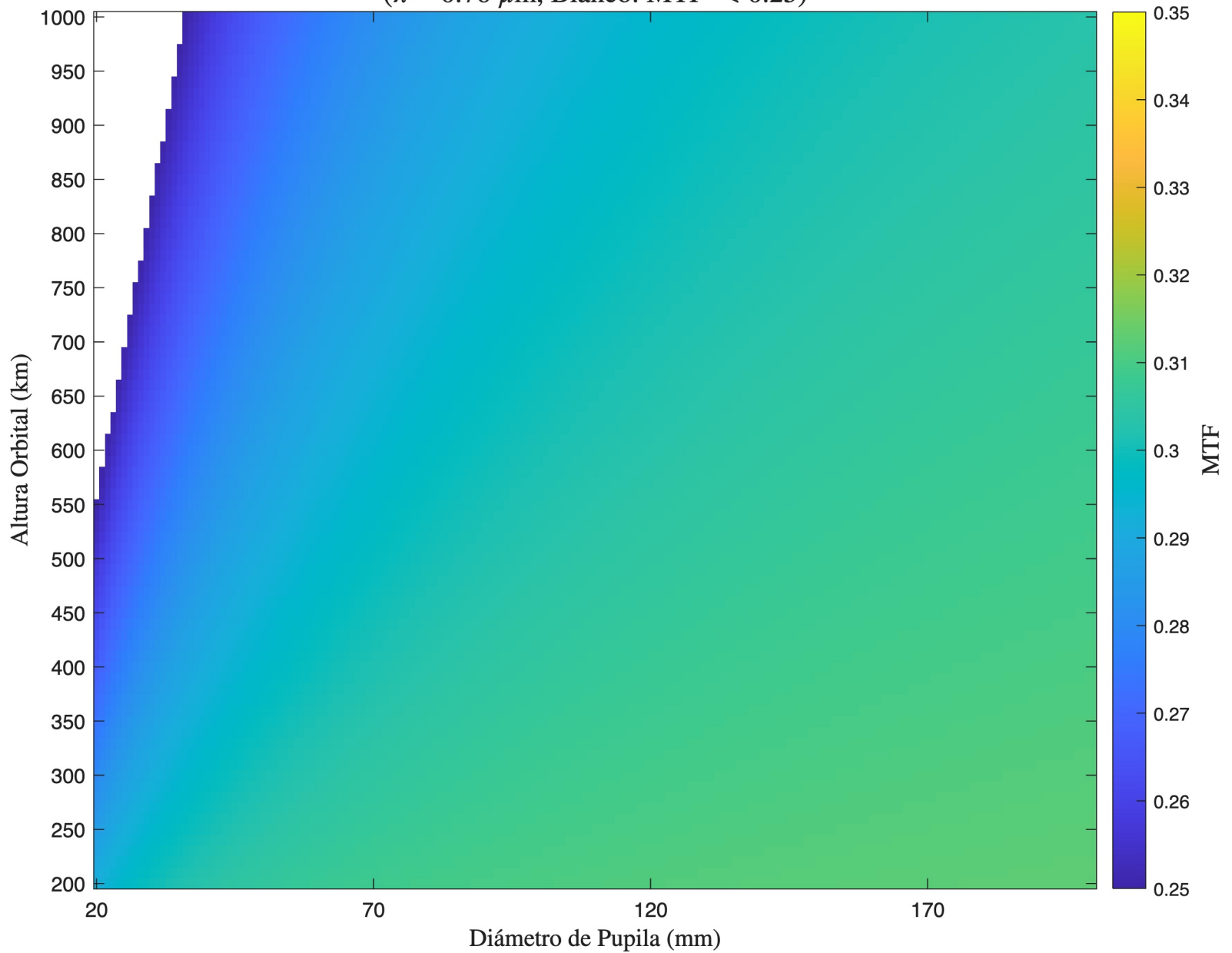
MTF - Cassegrain - Detector 2 ( \lambda = 0.76 \mu\text{m} , Blanco: MTF < 0.25)
