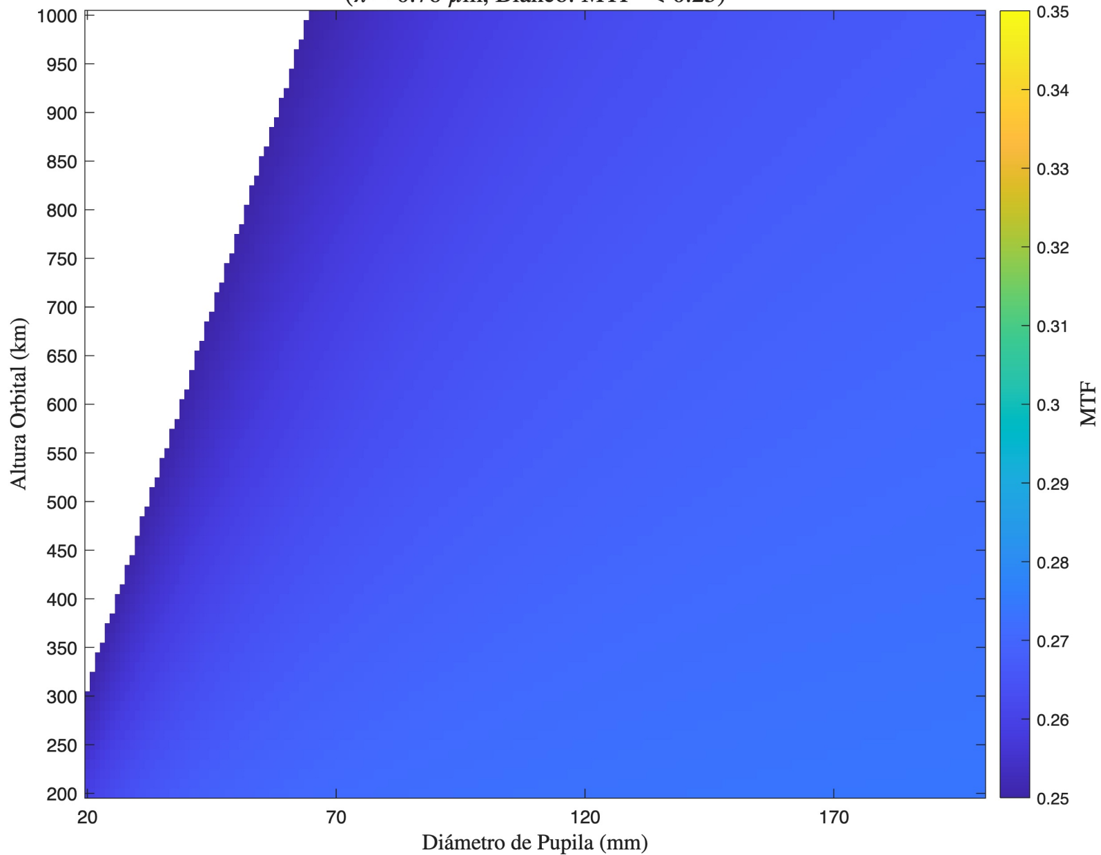
MTF - TMA - Detector 2 ( \lambda = 0.76 \mu\text{m} , Blanco: MTF < 0.25)
