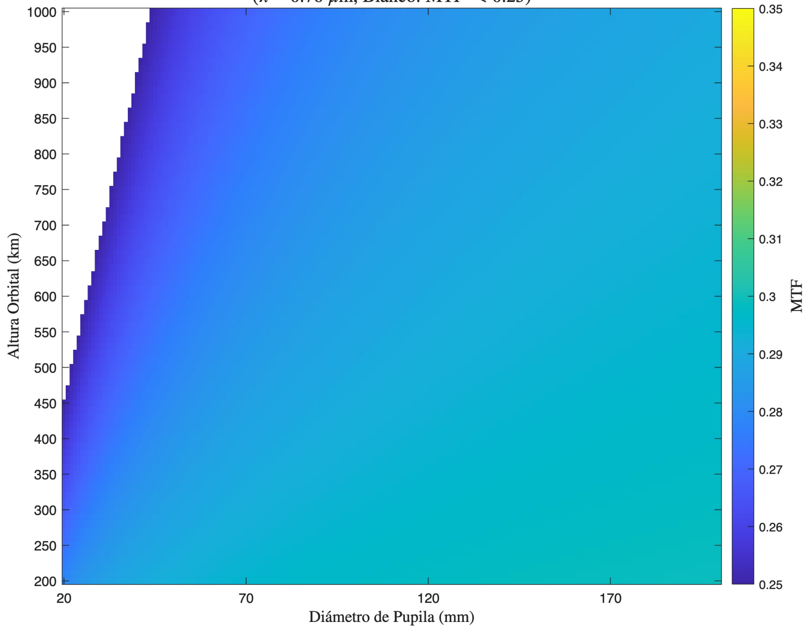
MTF - Korsch - Detector 3 ( \lambda = 0.76 \mu\text{m} , Blanco: MTF < 0.25)
