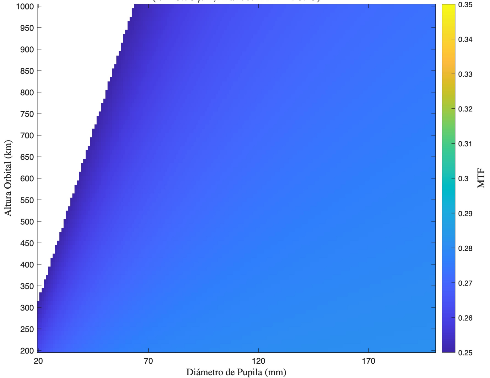
MTF - Cassegrain - Detector 3 ( \lambda = 0.76 \mu\text{m} , Blanco: MTF < 0.25)
