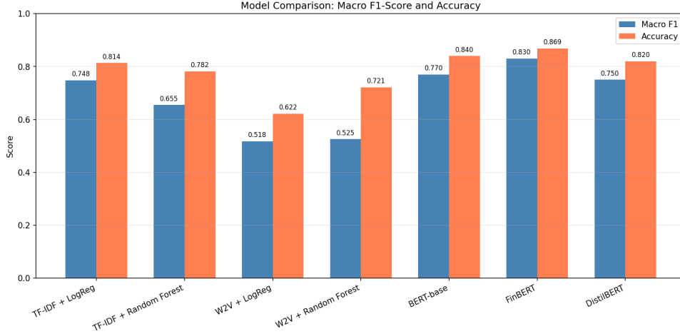
Figure 5: Macro F1-score comparison across all models.
