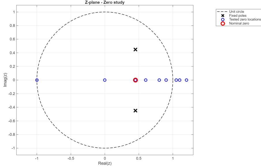
(a) Fixed poles and variable zeros.
