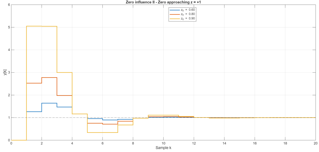
(b) Zero approaching z = 1 .
