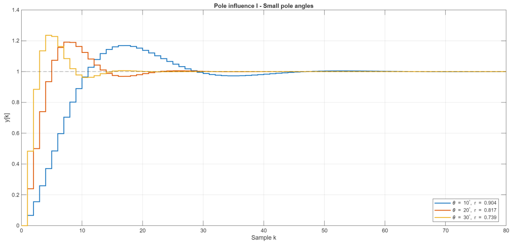
(a) Small pole angles.
