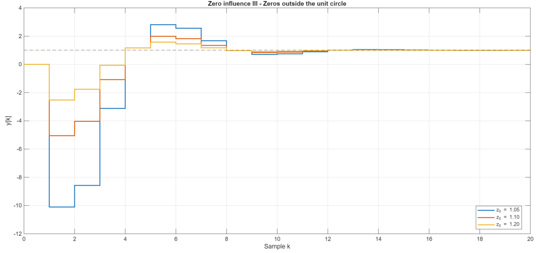
(c) Zeros outside the unit circle.
