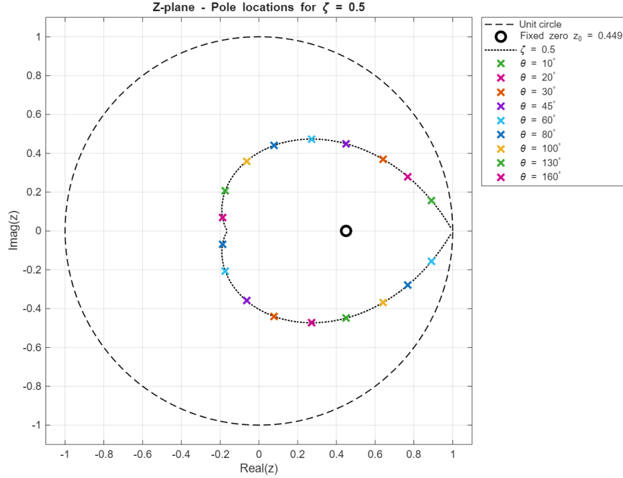
(b) Fixed zero and variable poles.
