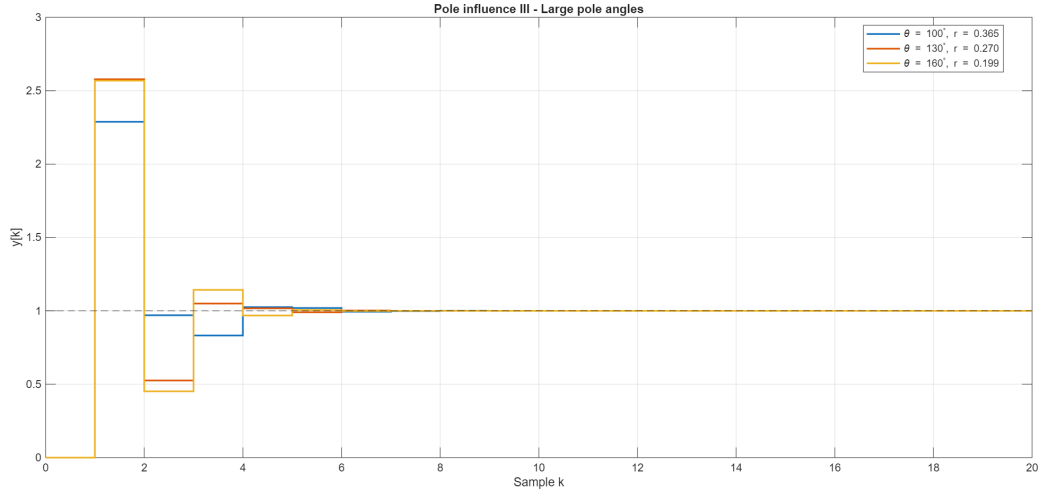
(c) Large pole angles.
