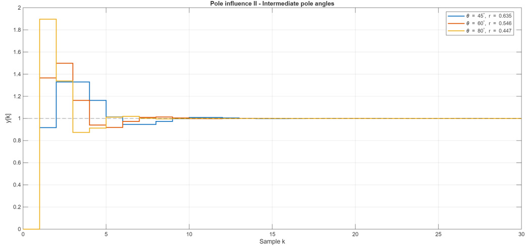
(b) Intermediate angles.
