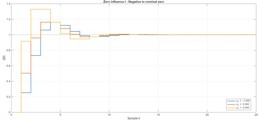
(a) Negative to nominal zero.
