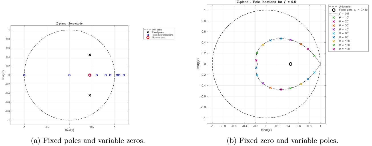
Figure 3: Pole-zero configurations used in the simulations.
