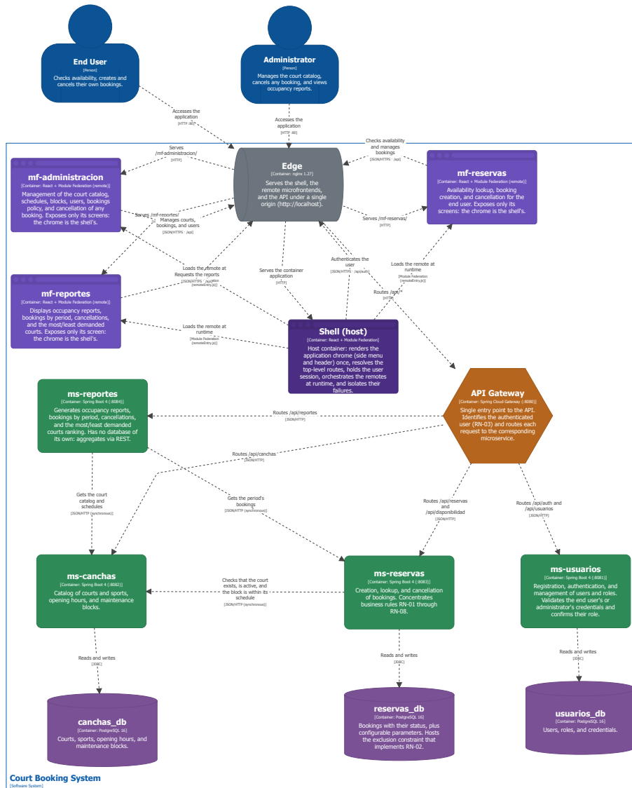
Container View: Court Booking System Level 2 — Microfrontends, gateway, microservices, and databases. Saturday, August 29, 2026 at 3:10 AM Ecuador Time
