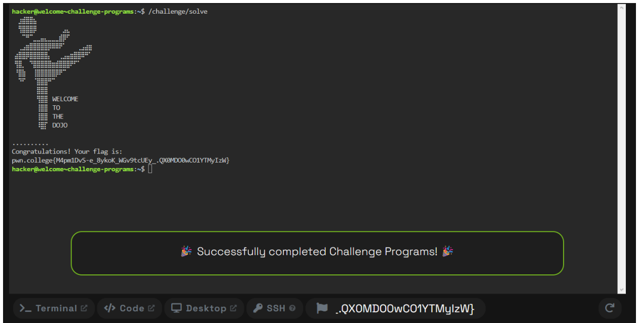
fig6. Challenge Programs
