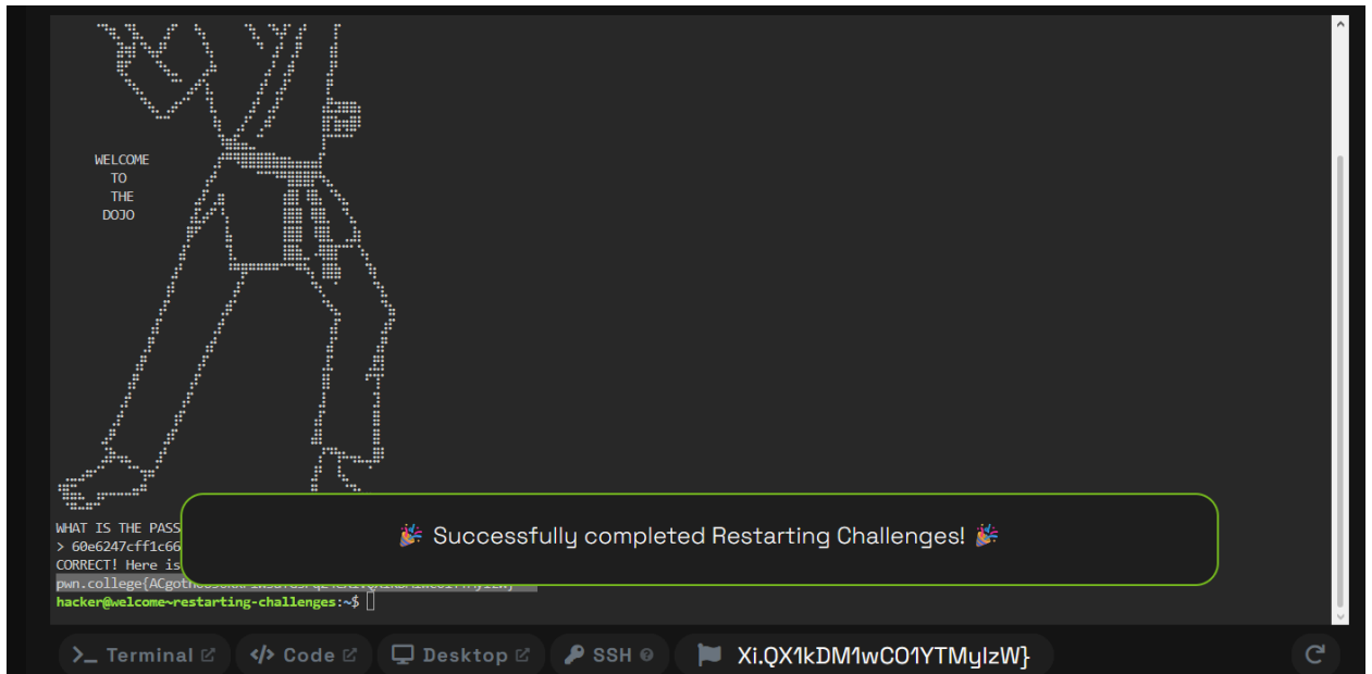
fig6. Challenge Programs
