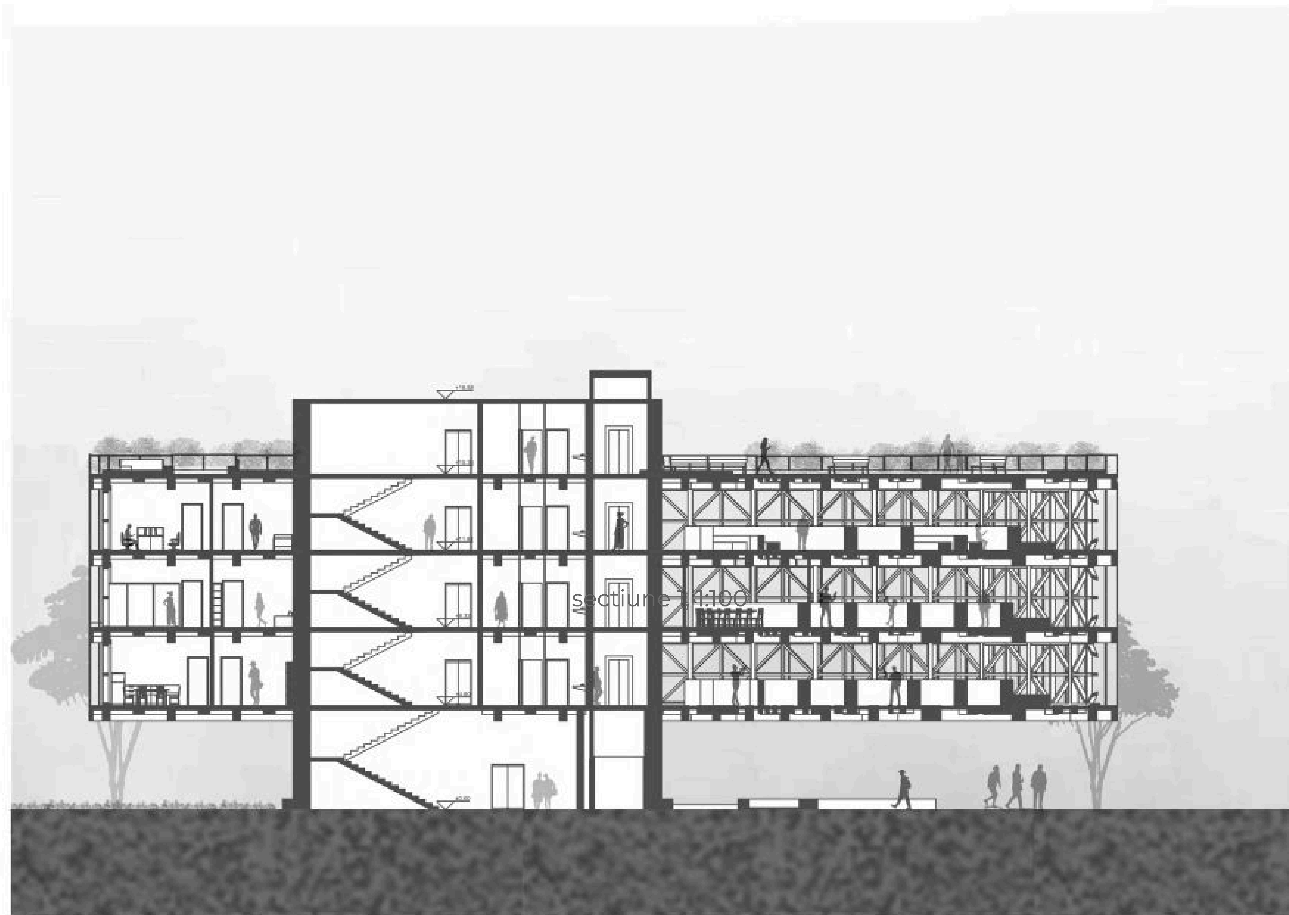
section 2, 1:100
