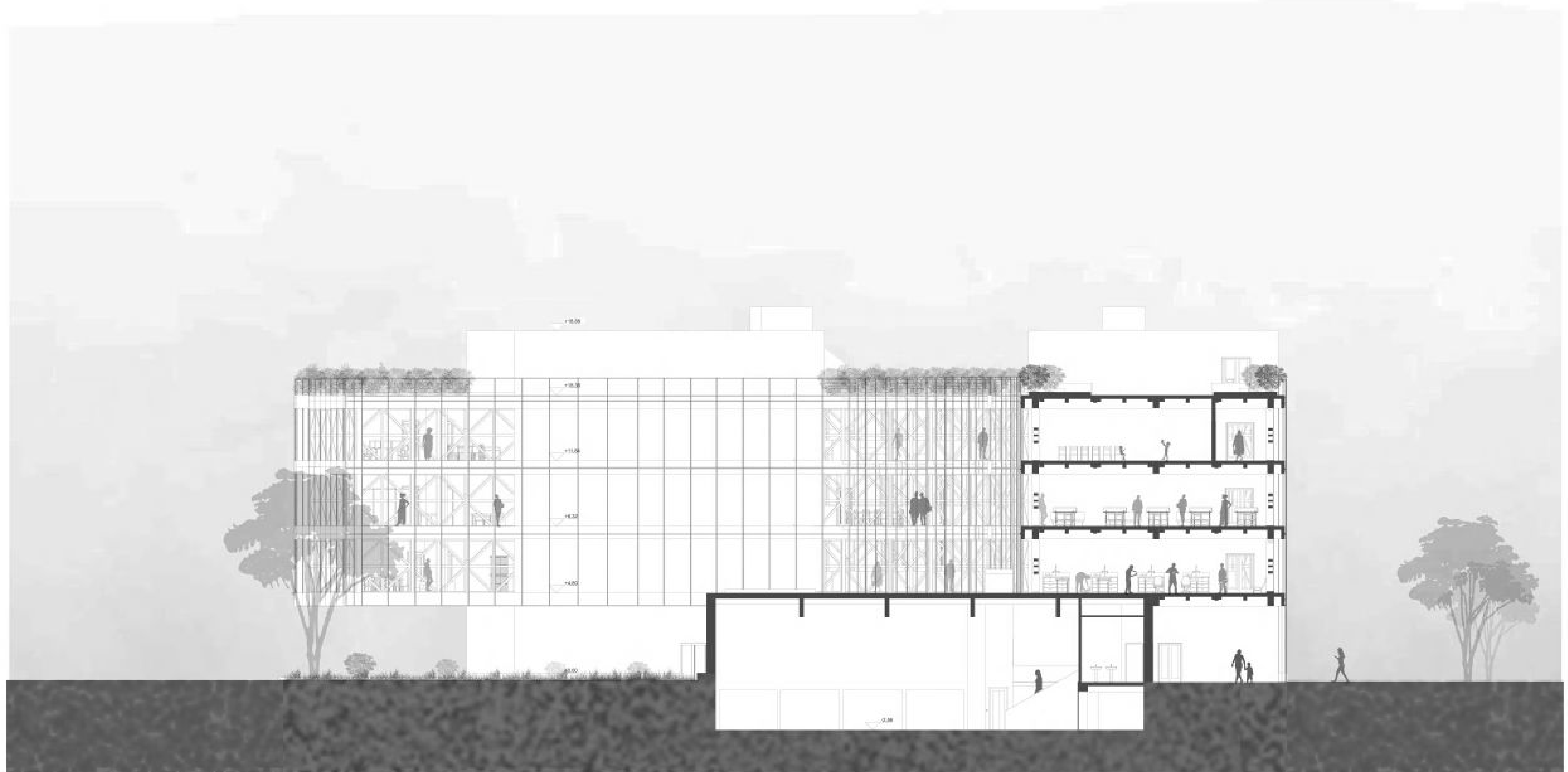
section 1, 1:100
