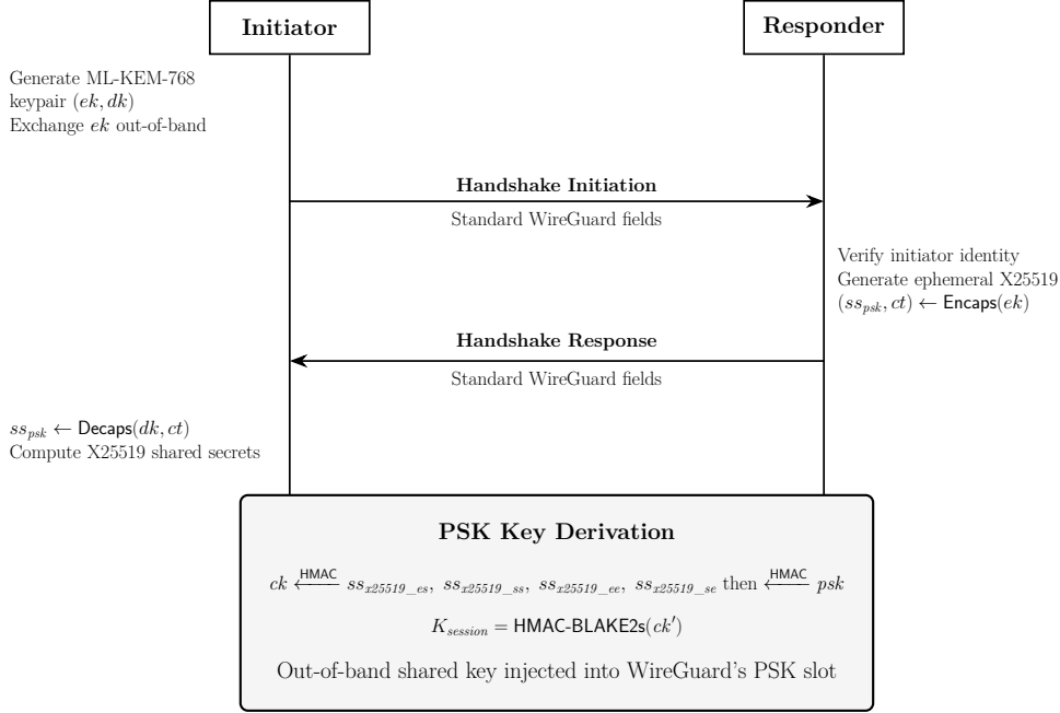
Figure 1: PSK-Slot baseline: out-of-band ML-KEM exchange and PSK injection.
