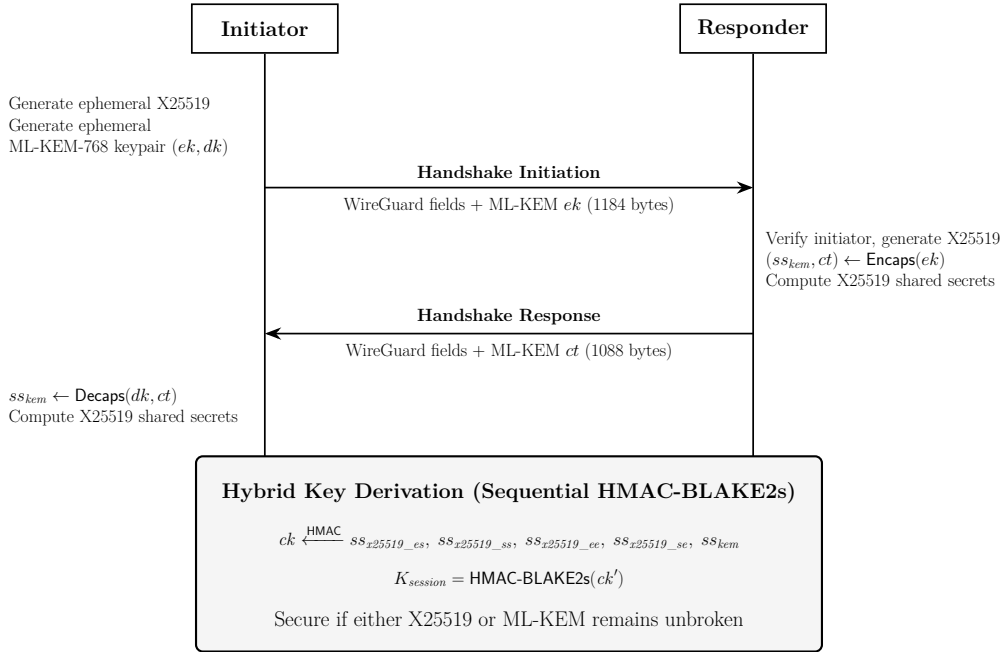
Figure 2: The full hybrid handshake: integrated ML-KEM-768 alongside X25519.
