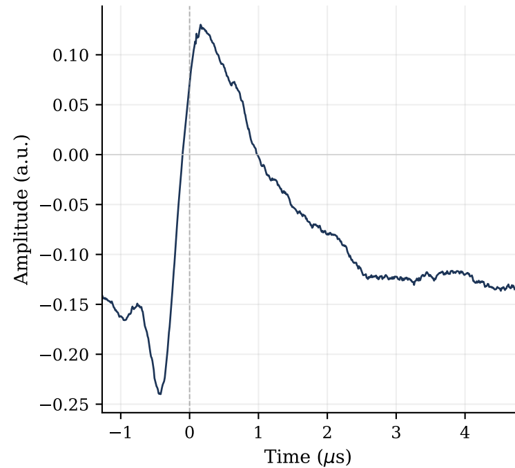
(a) Windowed time-domain pulse
