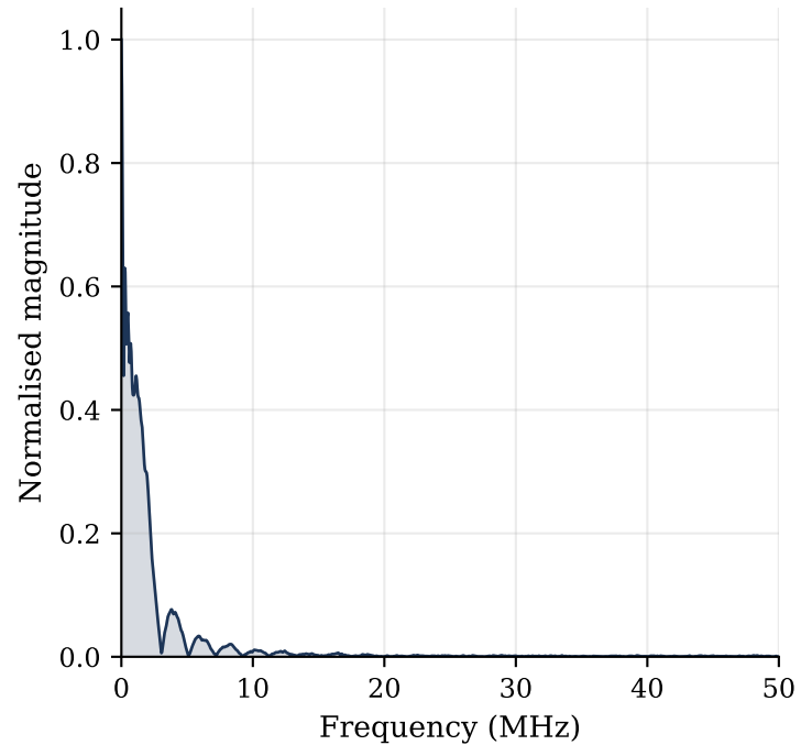
(b) Magnitude spectrum (FFT)
