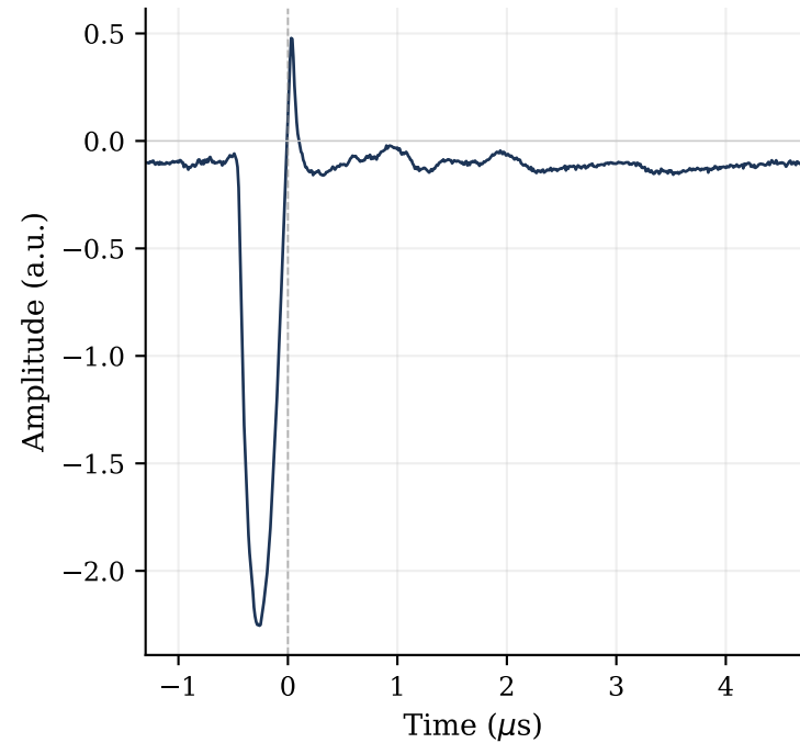
(a) Windowed time-domain pulse
