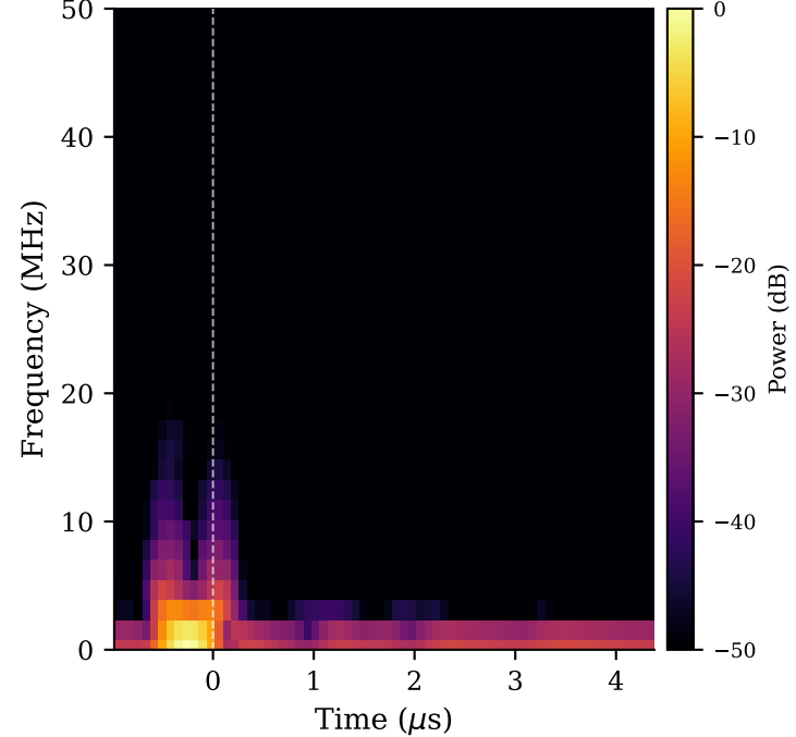
(c) Spectrogram (STFT)
