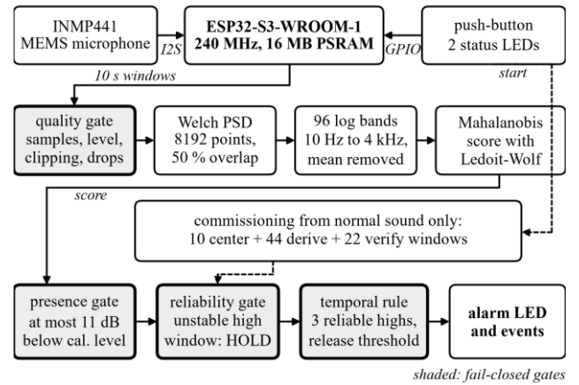
Fig. 1. Signal path and decision chain. Shaded blocks are fail-closed gates. Calibration, thresholds and alarms are computed on the device; the PC only logs telemetry and operator labels.
