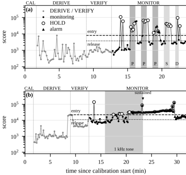
Fig. 2. Complete sessions on the physical fan, one point per 10 s window: (a) paper strip (P), speech (S) and door (D); (b) 1 kHz tone. Shading follows operator labels, not independently measured stimulus boundaries; the tone continued beyond its shaded block. Thresholds come from DERIVE. Unconfirmed windows are excluded from Table II.
