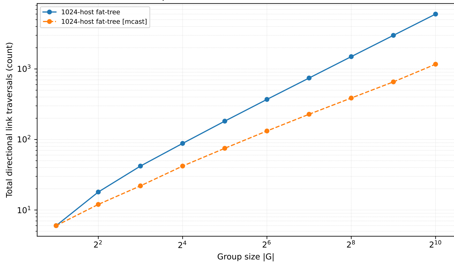
Network footprint: baseline vs multicast (1024-host fat tree)
